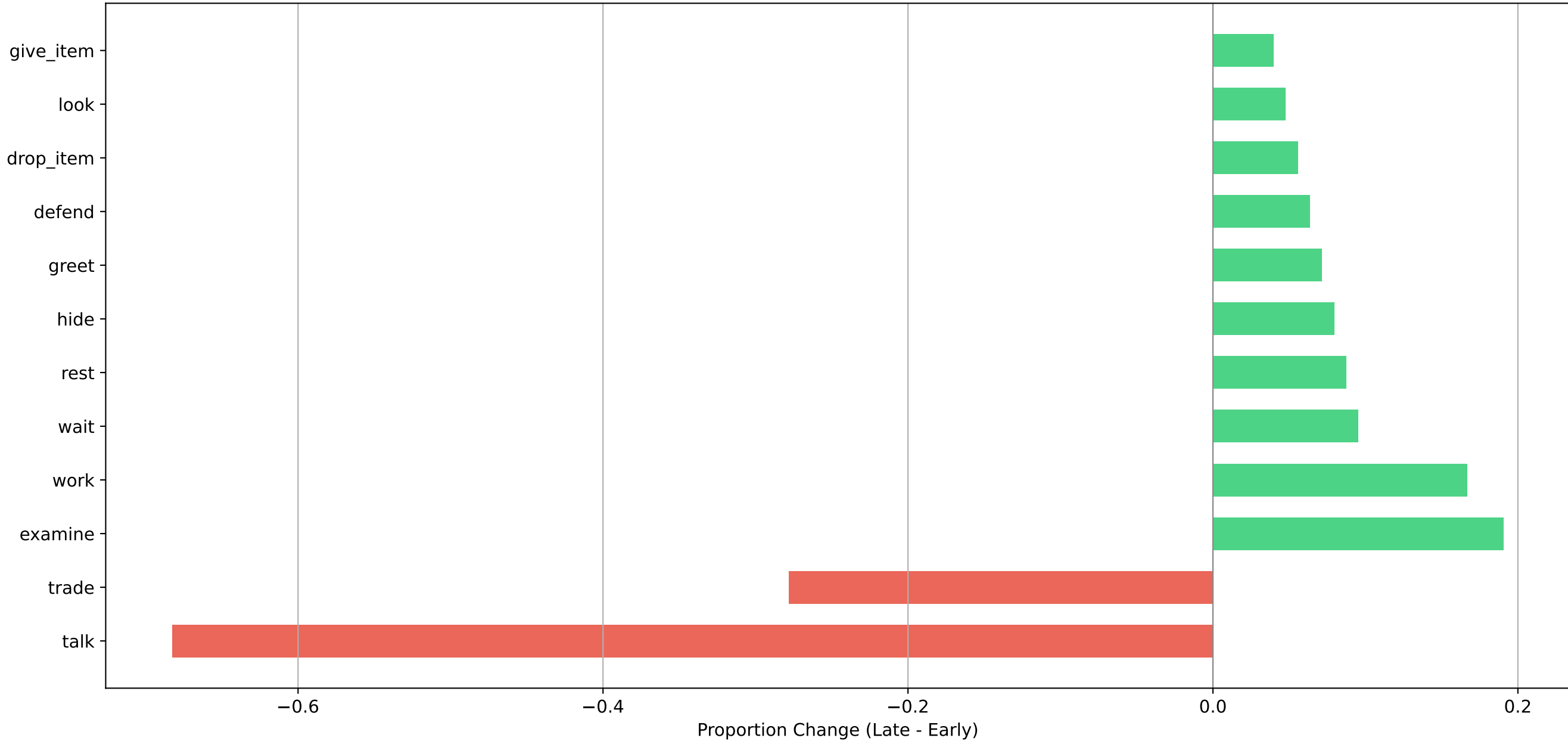
NPC Action Distribution Shift: Early vs Late Game (C1)
