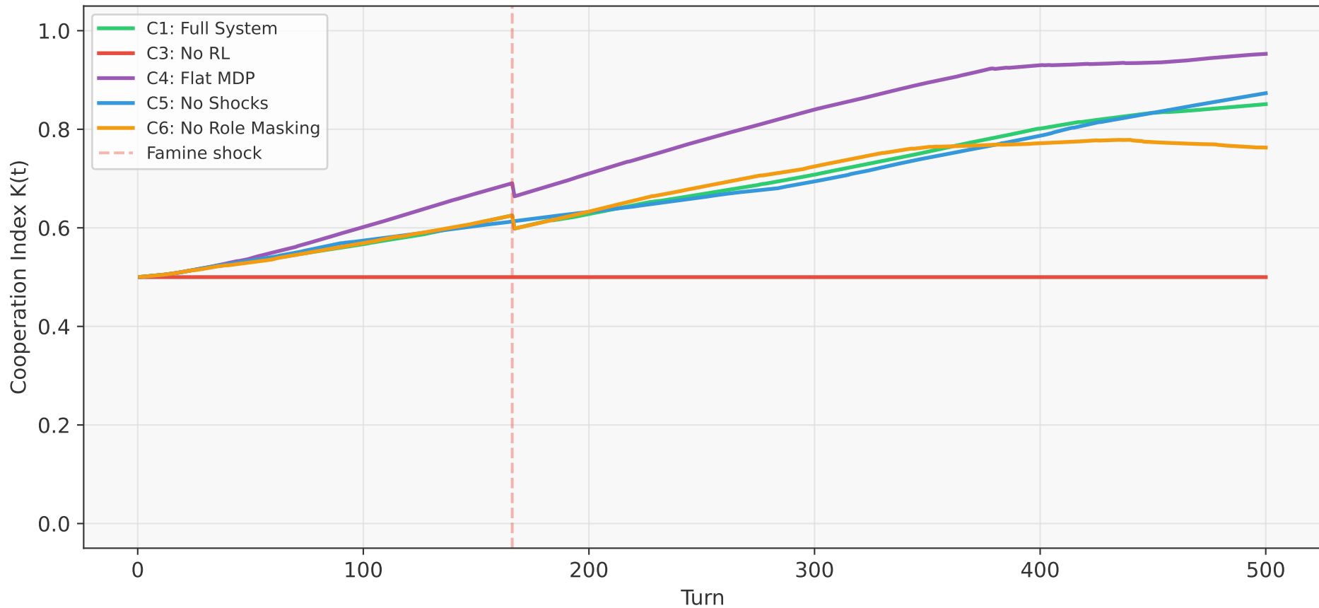
Cooperation Emergence: Ablation Comparison
