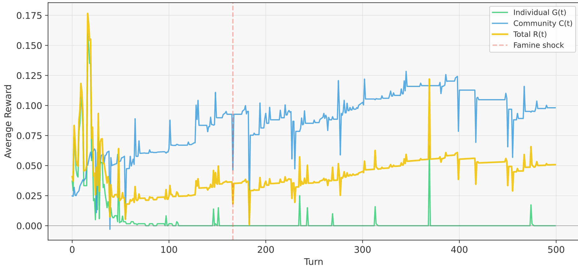
Reward Decomposition (C1: Full System)
