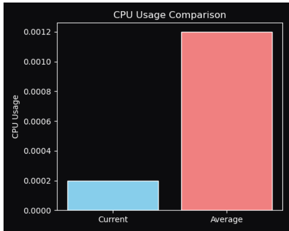
Cpu
