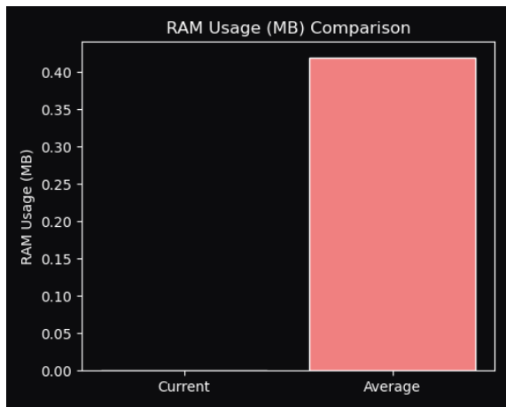
Ram
