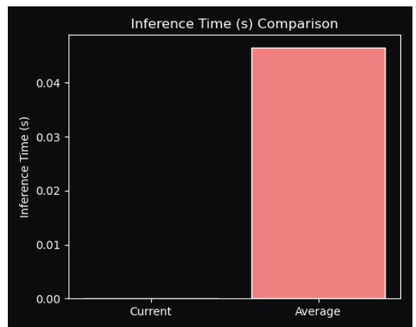
Inference time
