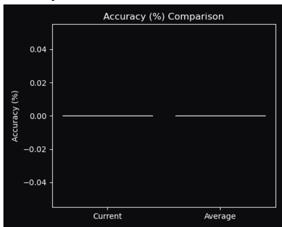
Accuracy
