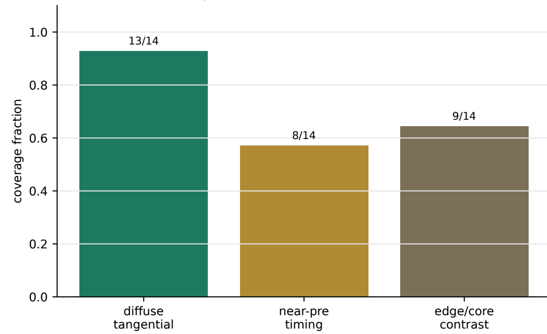
D. Repeated form and bounded structure
