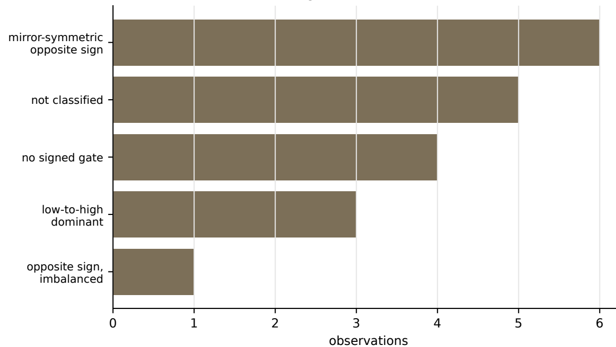
C. Signed structure classes
