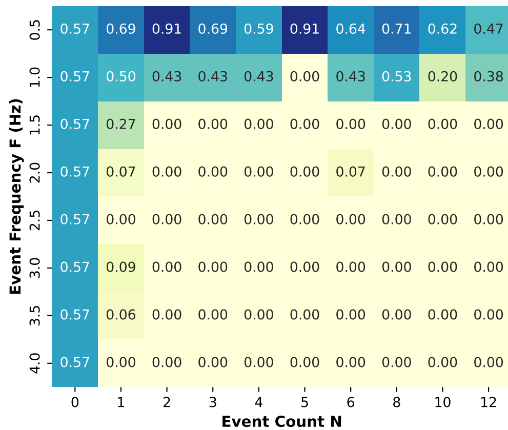
Prompt: Thinking / CoT
