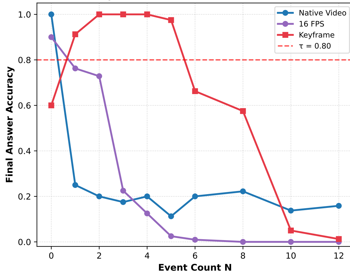
B. Keyframe Evidence vs Native & 16 FPS
