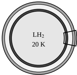
(a) Section, gap exaggerated
