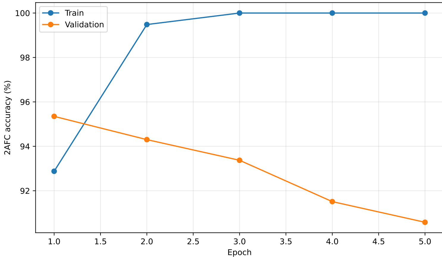
Training and validation 2AFC accuracy
