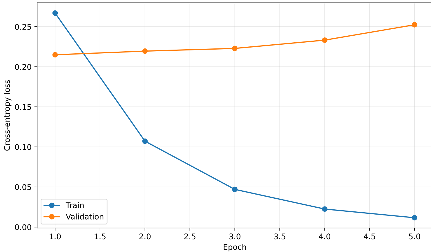
MoH training and validation loss
