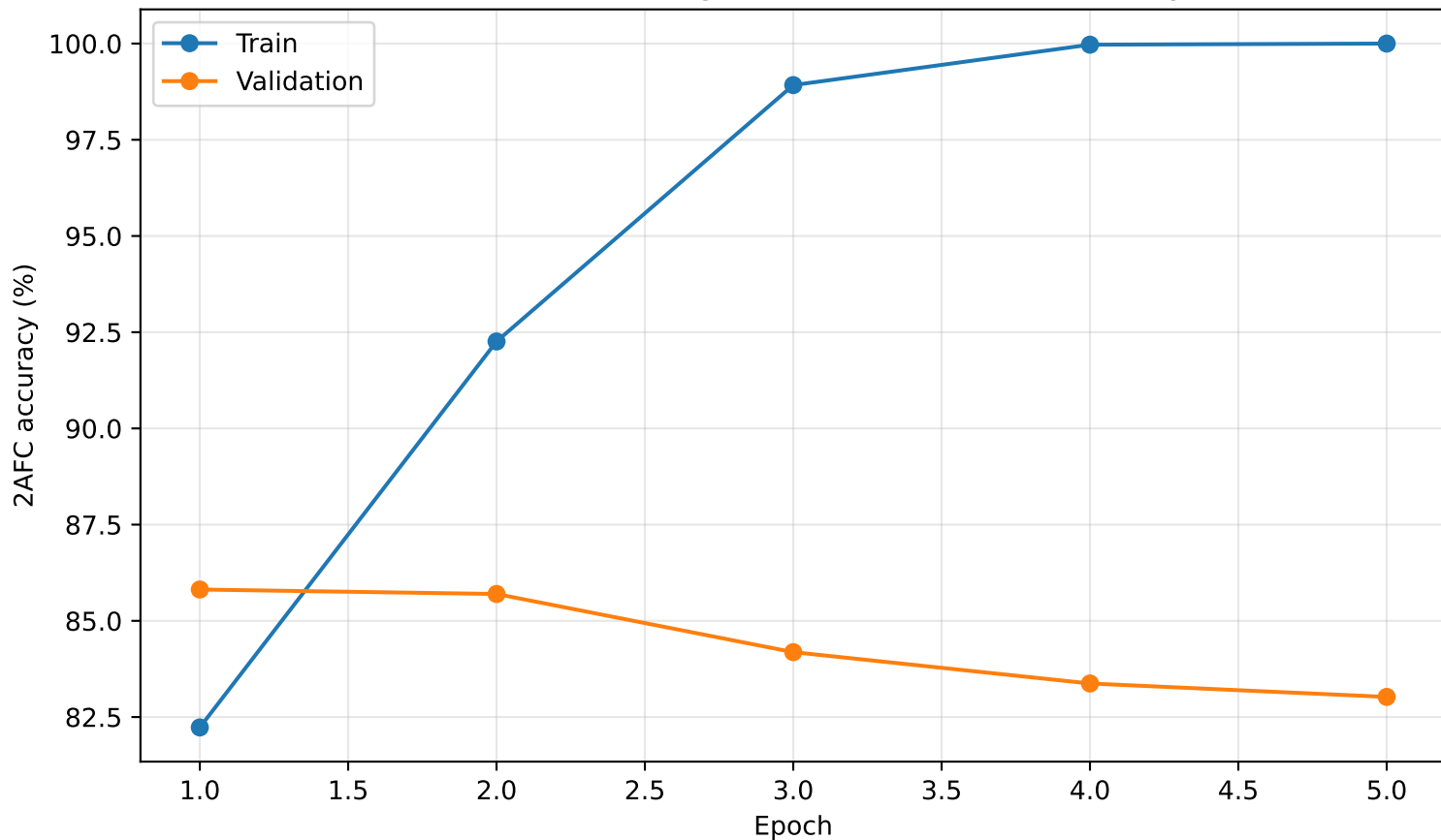
MetaFormer training and validation 2AFC accuracy
