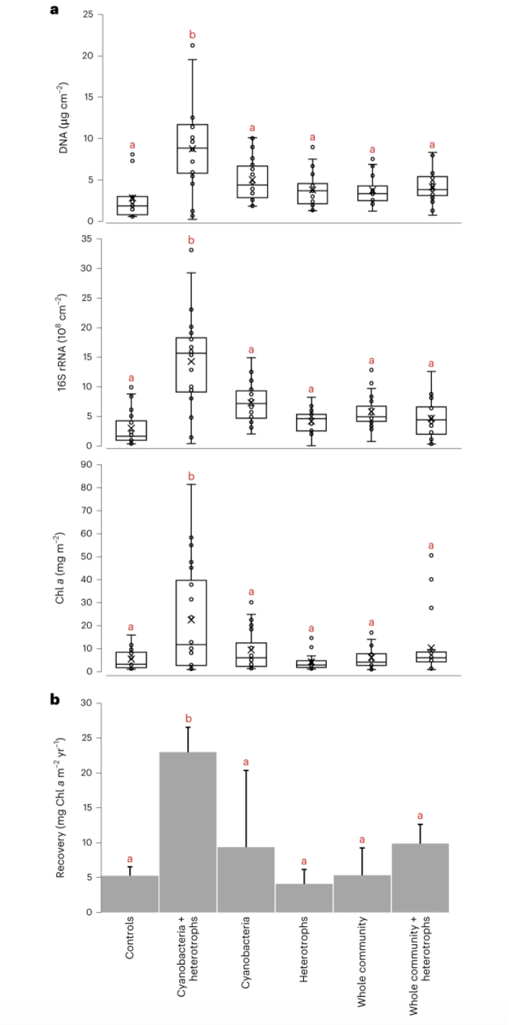
Fig. 5: Effect of inoculum type on end-point biocrust development and recovery rates.
