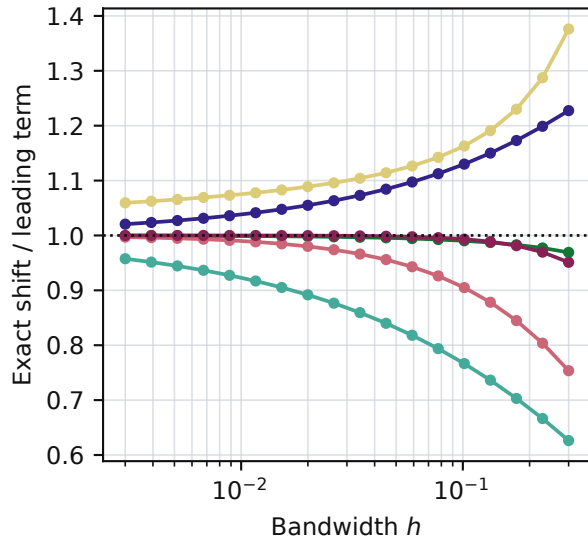
Coefficient convergence
