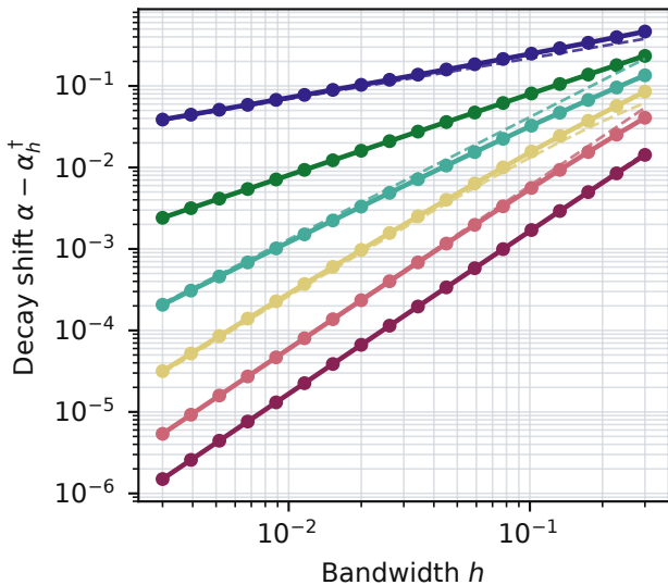
Exact shift and leading term
