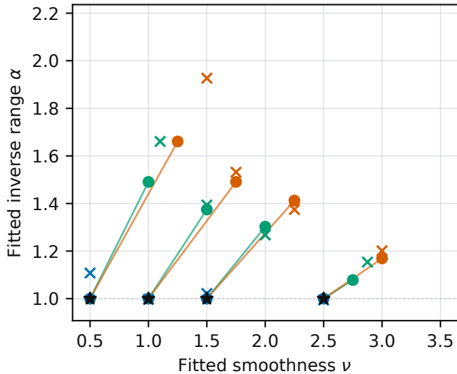
True bandwidth h = 0.35
