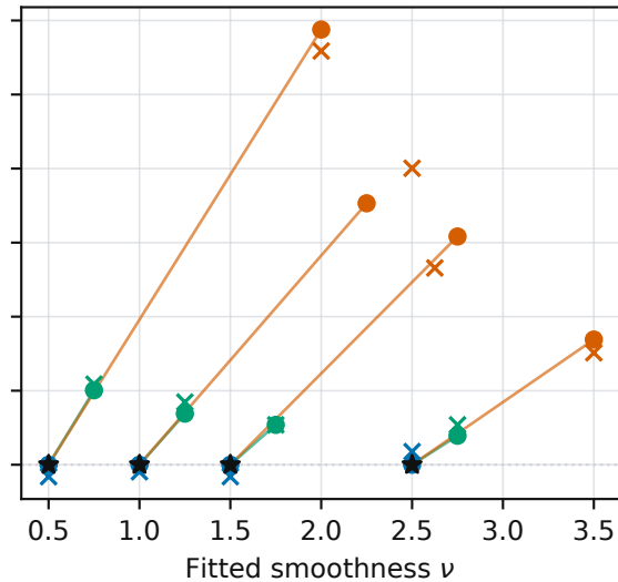
True bandwidth h = 0.5
