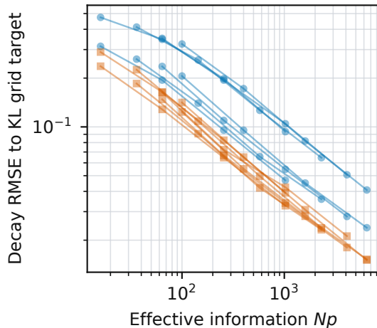
Stochastic error contracts
