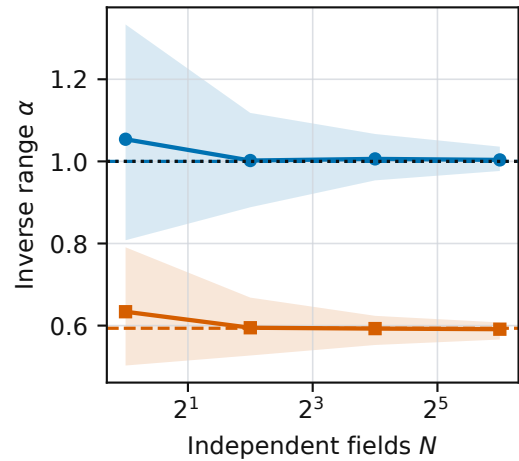
More precise, wrong target ( p = 100, \nu = 1.5 )
