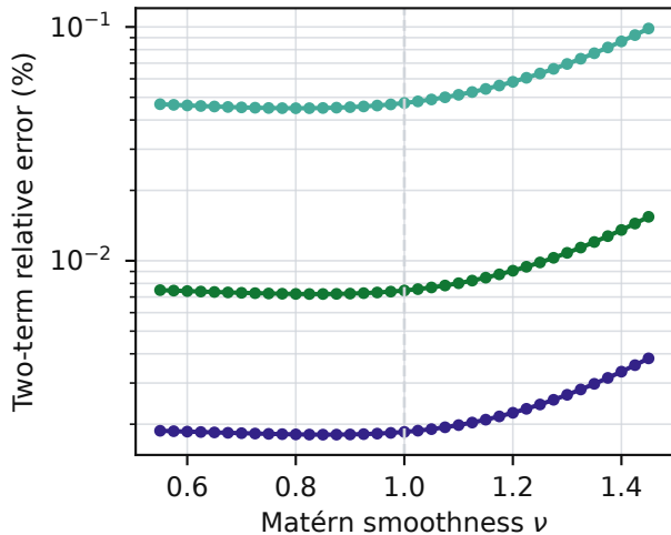
Cancellation-aware approximation
