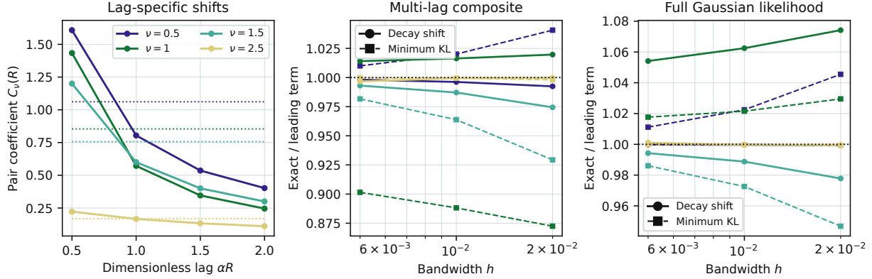
Genuine likelihood misspecification has the predicted local geometry
