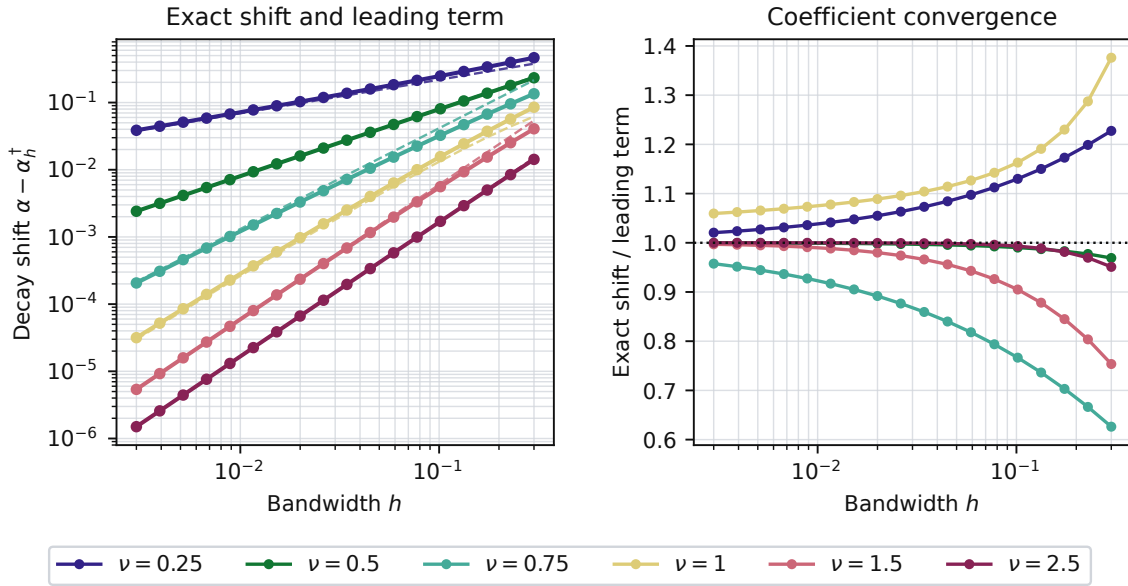
Figure 1: Continuous two-dimensional pseudo-decay shift. Left: exact shifts (solid) and theorem leading terms with explicit coefficients (dashed). Right: their ratio, which approaches one as h \downarrow 0 .
