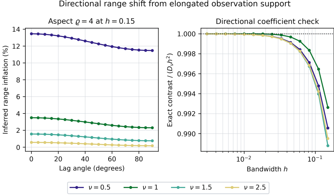
Figure 4: An isotropic latent field observed through elongated support. Left: apparent range inflation versus lag angle at support aspect four and h = 0.15 . Right: exact major–minor inverse-range contrast divided by D_v h^2 .
