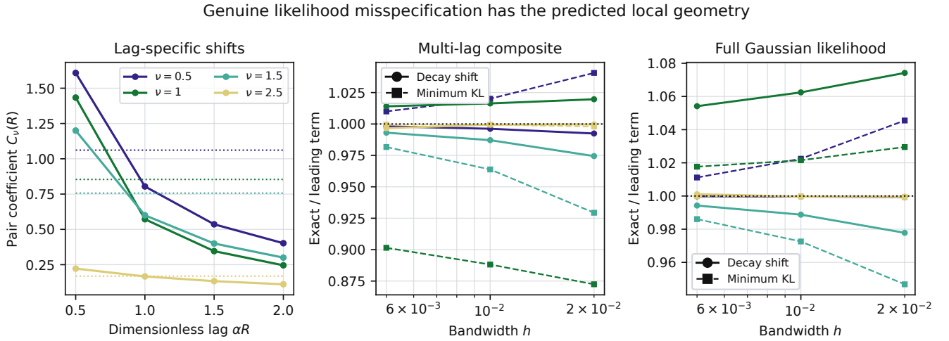
Figure 3: From a saturated pair match to genuine misspecification. Dotted segments in the left panel are the information-weighted composite coefficients. The middle and right panels validate both the pseudo-parameter shift and the first nonzero minimum-KL term.
