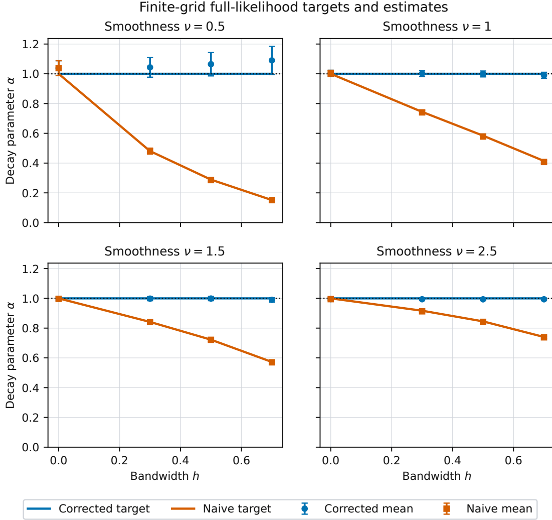
Figure 3: Finite-design full-likelihood targets and Monte Carlo mean estimates. Error bars show two Monte Carlo standard errors of the mean.
