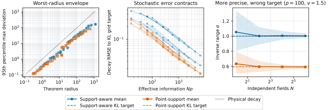
Figure 5: High-dimensional SupportShift likelihood benchmark. Left: the weaker worst-radius envelope; exact candidatewise coverage is reported in text. Center: decay RMSE to each model’s finite-grid KL target versus Np . Right: increasing N makes both estimators more precise, but the point-support fit concentrates near its displaced target.
