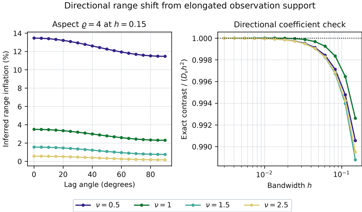
Figure 2: An isotropic latent field observed through elongated support. Left: apparent range inflation versus lag angle at support aspect four and h = 0.15 . Right: exact major-minor inverse-range contrast divided by D_v h^2 .
