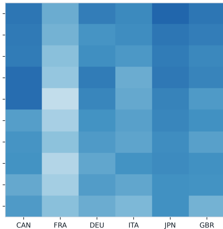
Leave-one-country-out alpha
