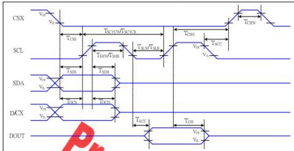
Figure 5-4-1: SPI serial Interface Timing Characteristics
