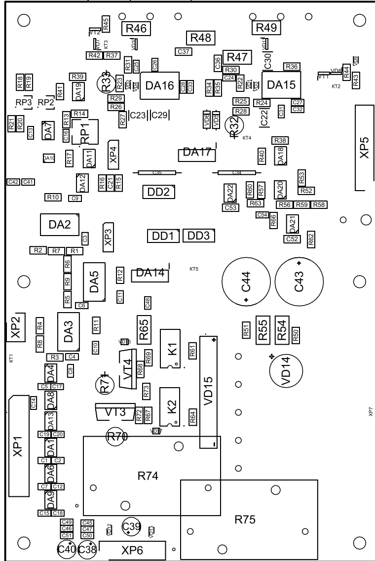
View from Top side (Scale 1:1)
