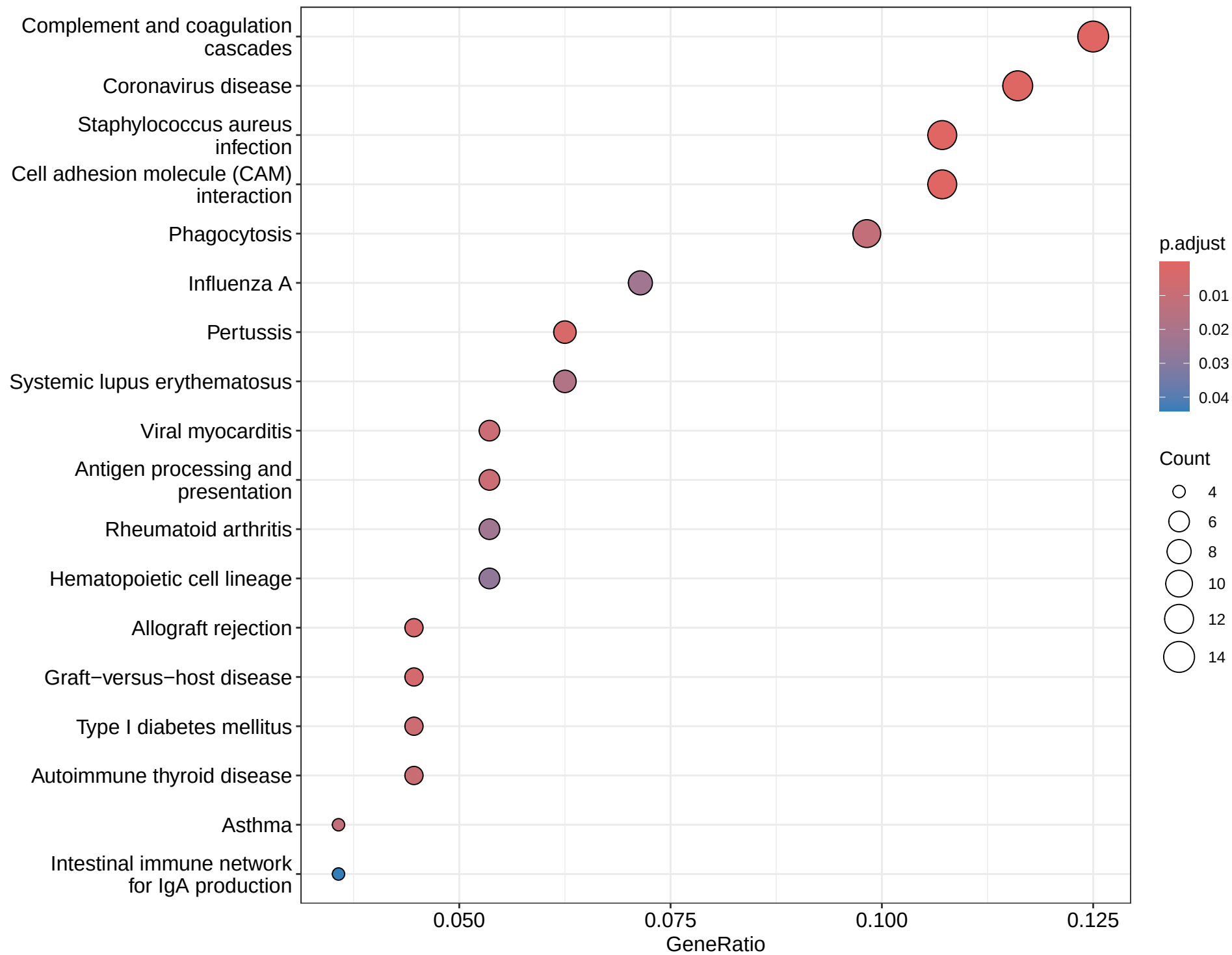
Intersection DEGs (182): KEGG pathways
