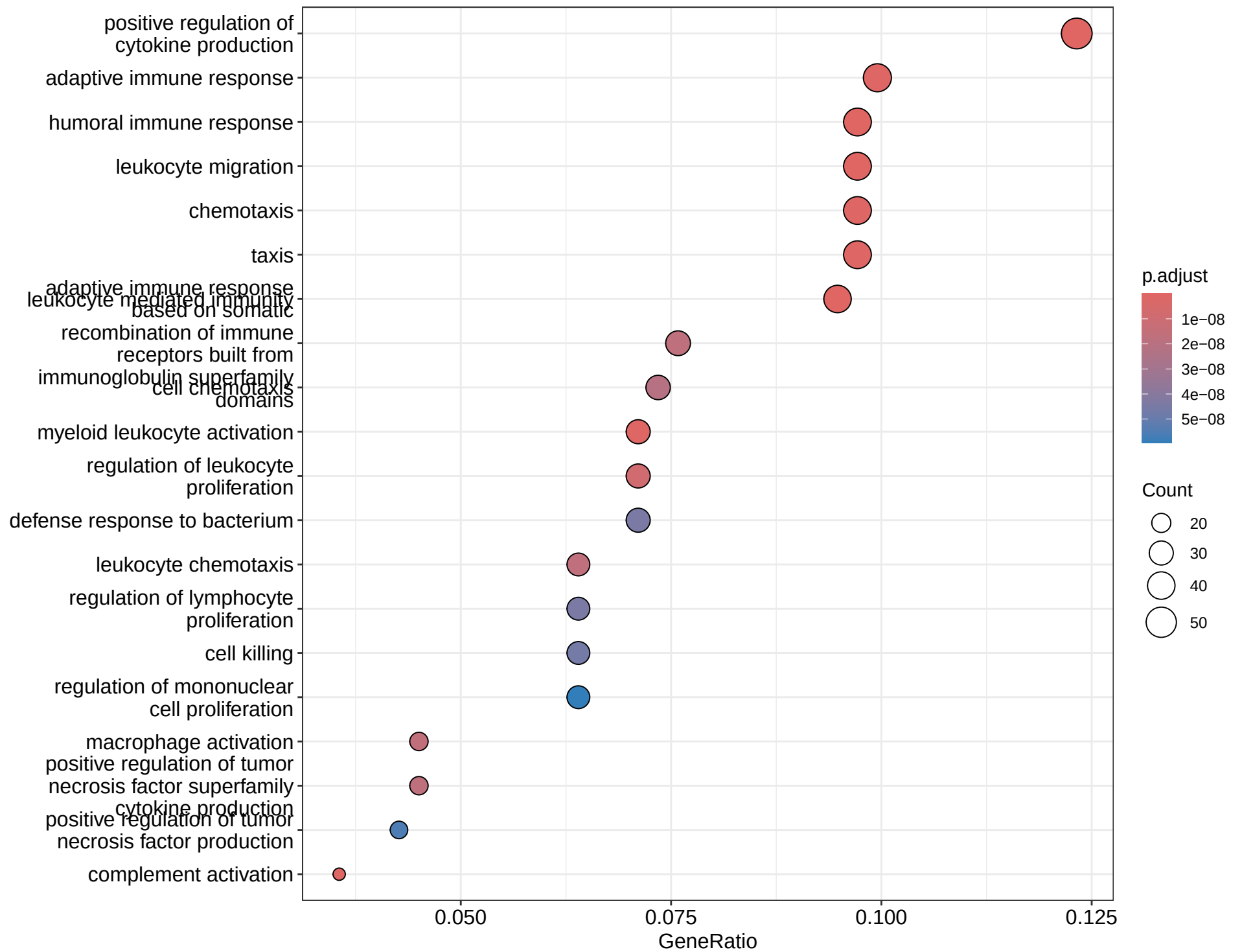
Full DEGs (447): GO Biological Process
