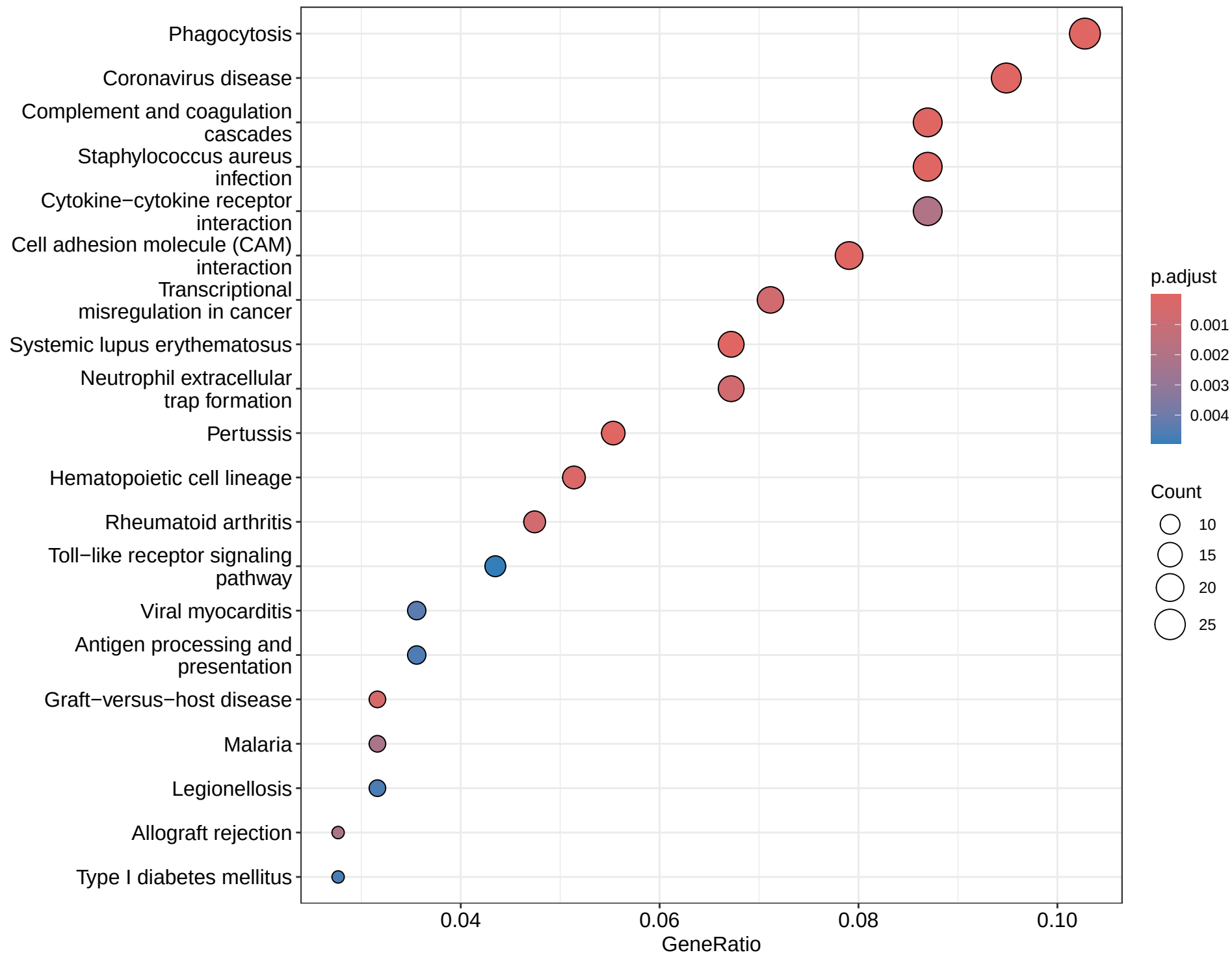
Full DEGs (447): KEGG pathways
