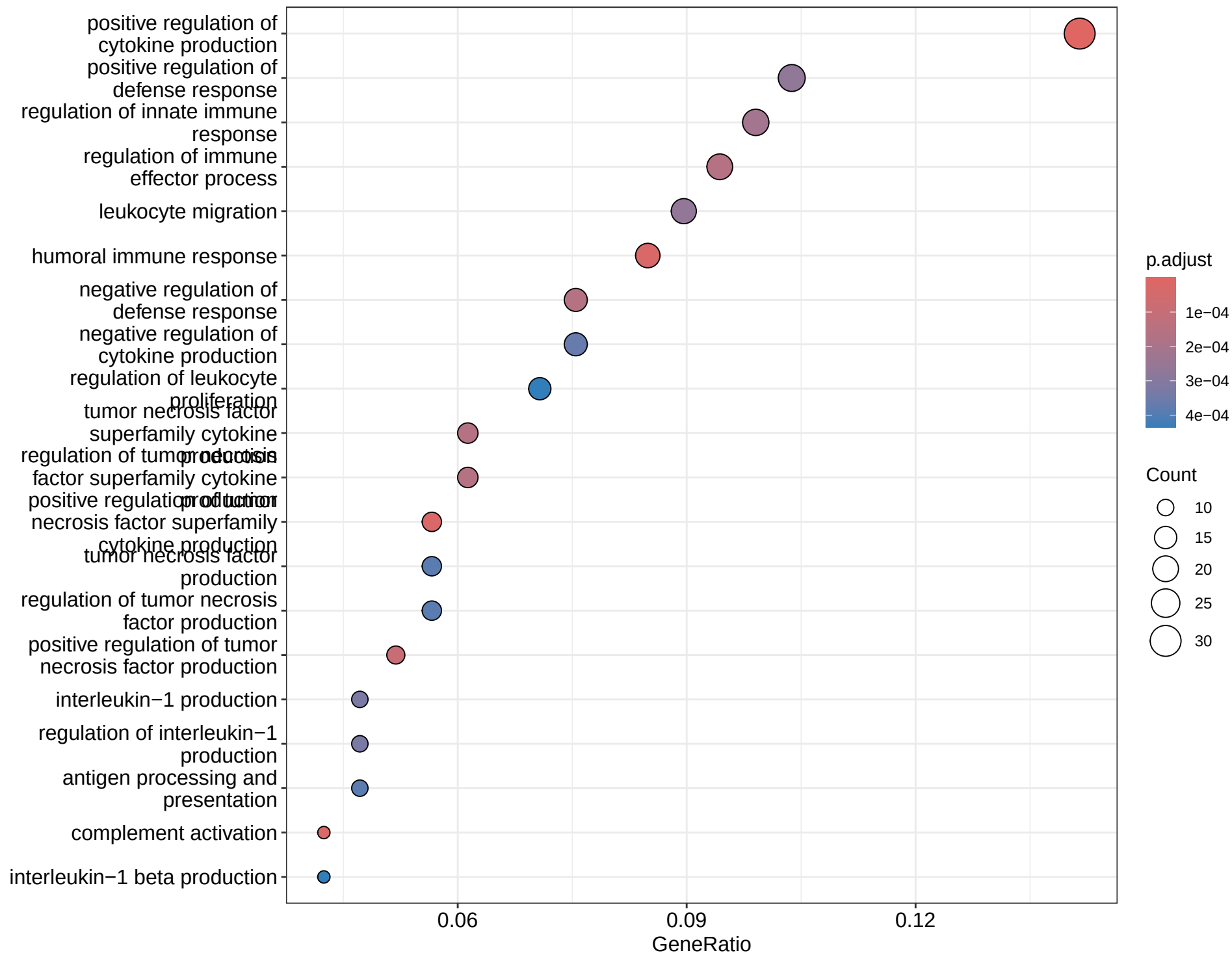
Intersection DEGs (221): GO Biological Process
