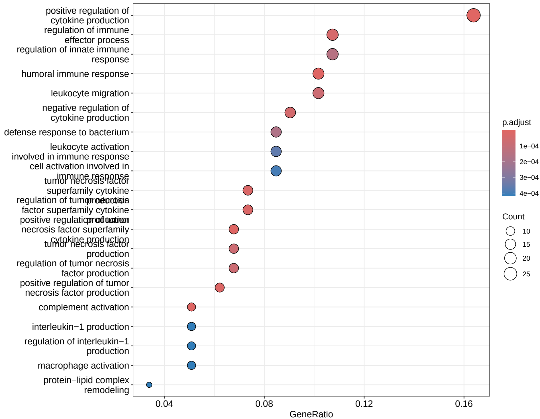
Intersection DEGs (182): GO Biological Process
