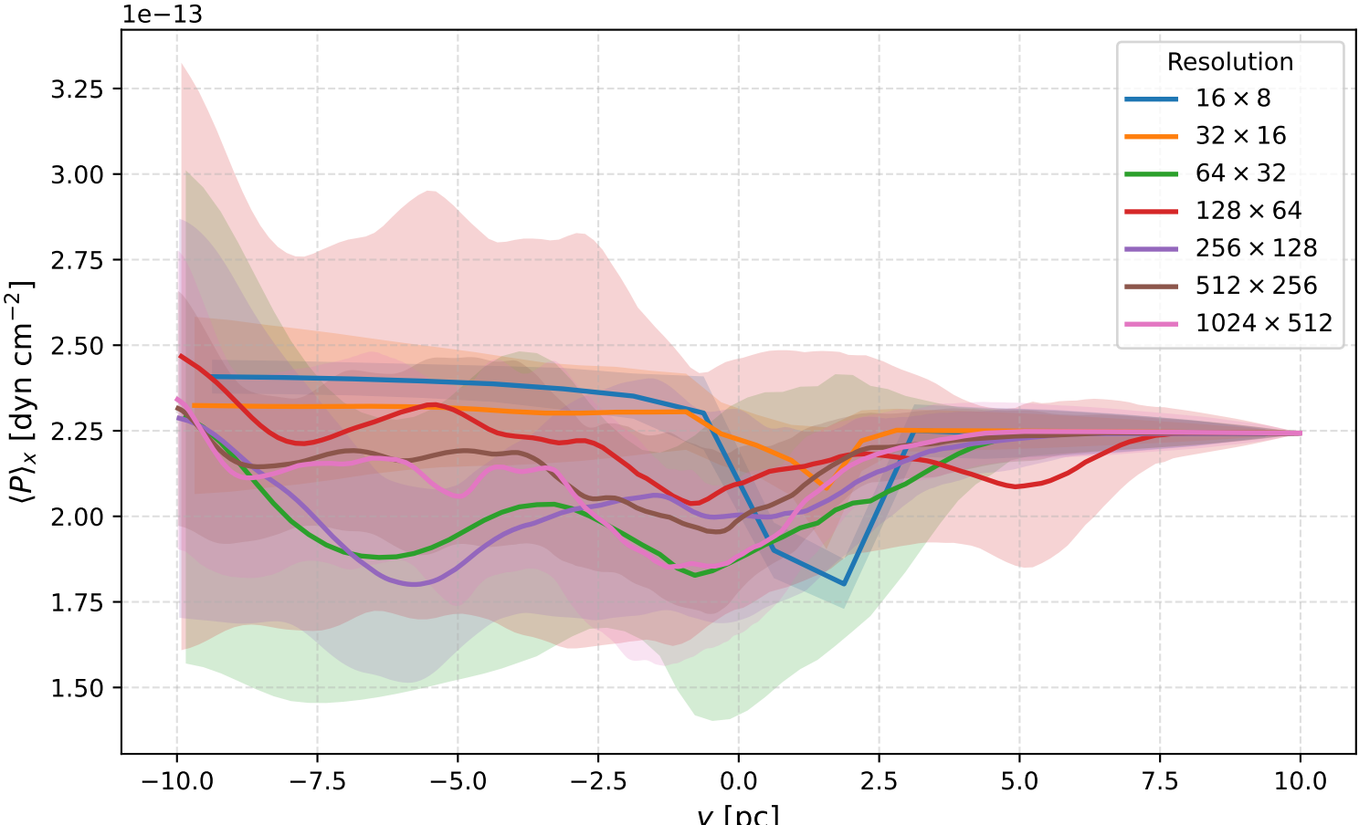
Pressure Profile \langle P \rangle_x (Time-averaged over last 500 snapshots, showing mean \pm 1\sigma across time)
