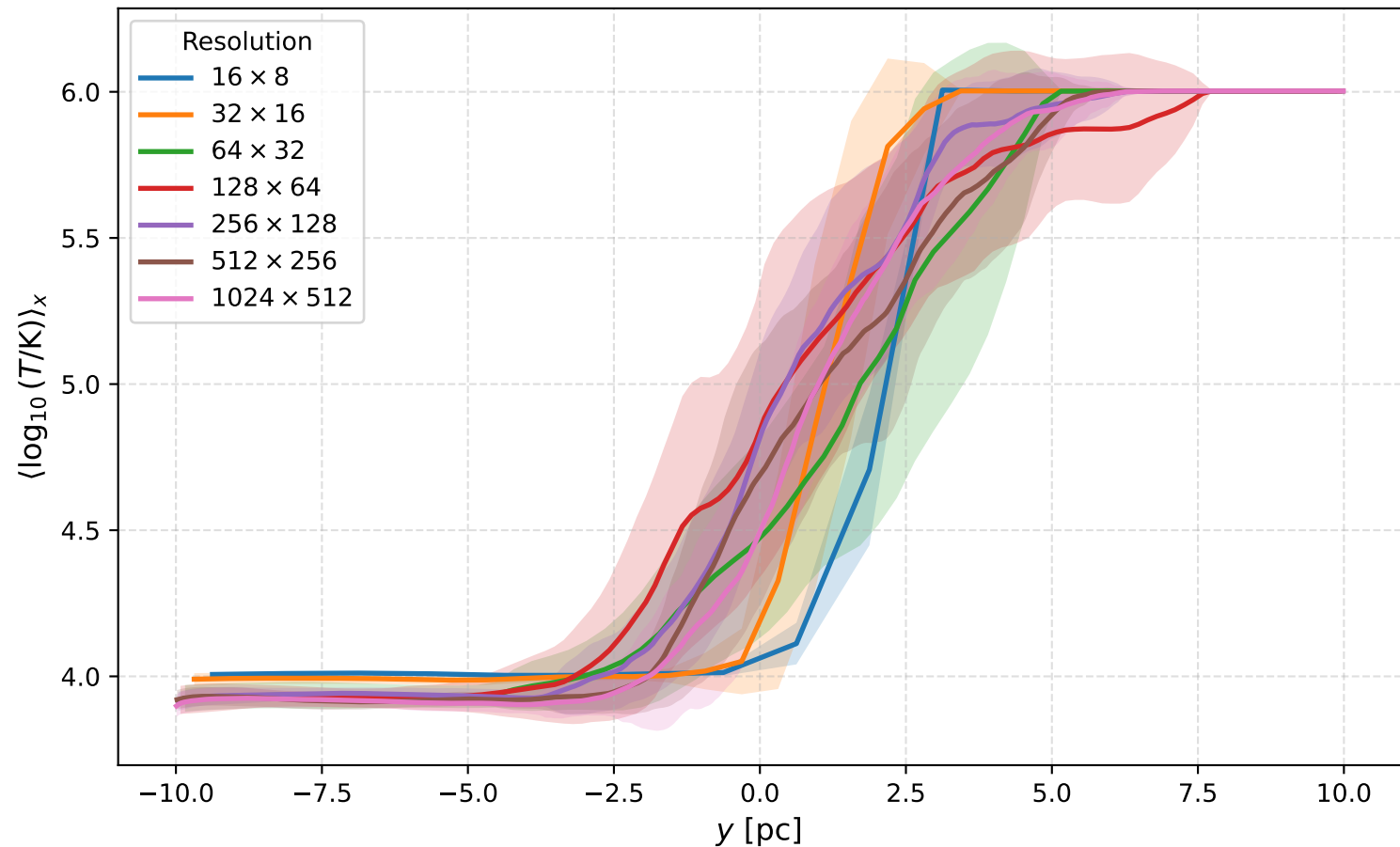
Log-Temperature Profile \langle \log_{10} T \rangle_x (Time-averaged over last 500 snapshots, showing mean \pm 1\sigma across time)
