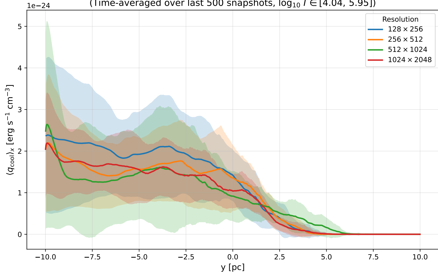
Mean Cooling Rate Profile vs y for HR MPI Simulations (Time-averaged over last 500 snapshots, \log_{10} T \in [4.04, 5.95] )
