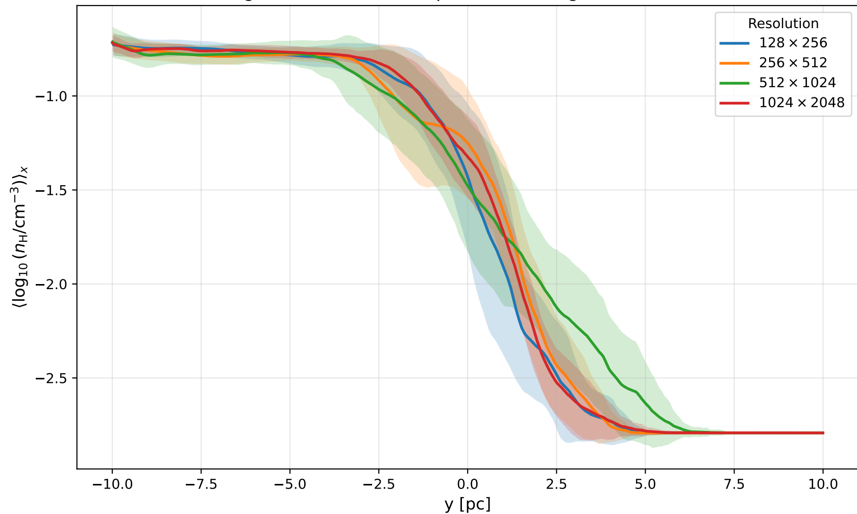
Log-Number-Density Profile \langle \log_{10} n_{\text{H}} \rangle_x (Time-averaged over last 500 snapshots, showing mean \pm 1\sigma across time)
