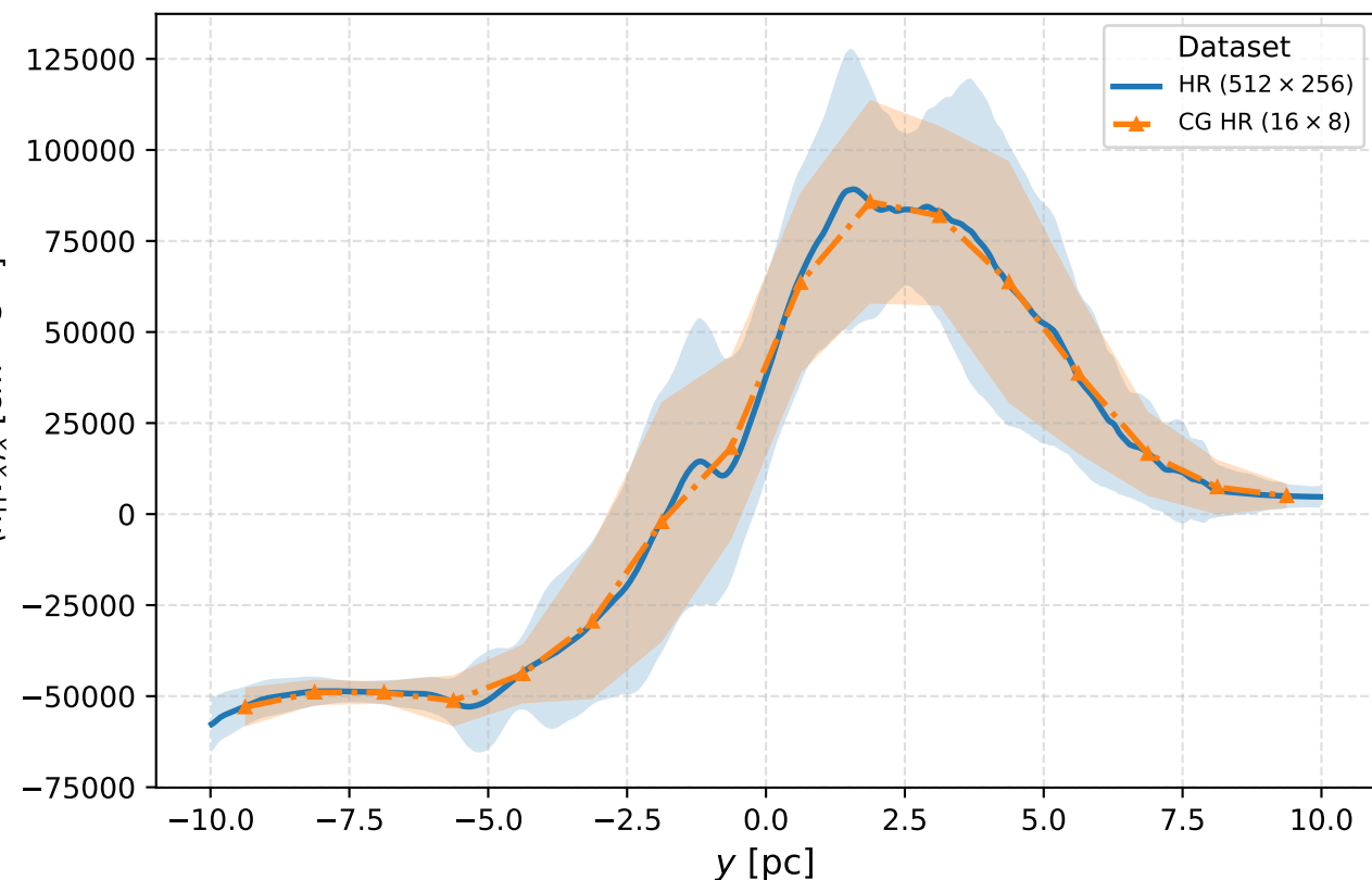
Horizontal Flux Profile \langle n_H v_x \rangle_x
