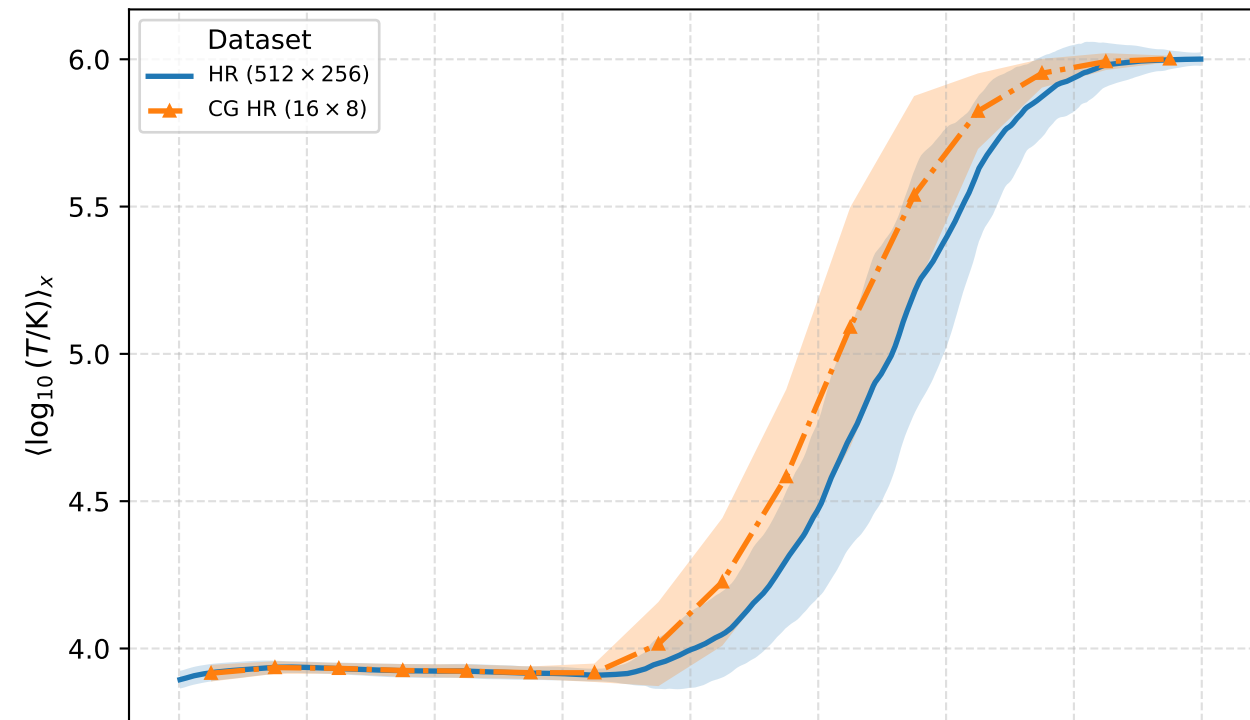
Log-Temperature Profile \langle \log_{10} T \rangle_x
