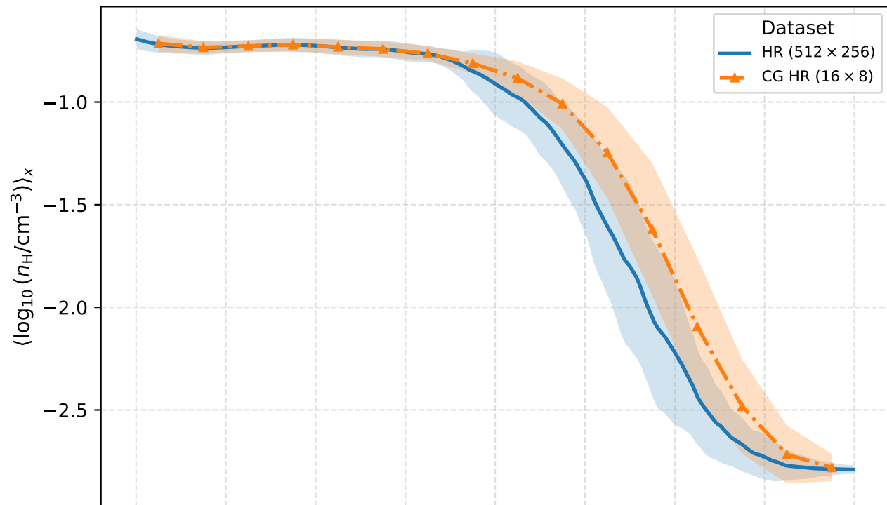
Log-Number-Density Profile \langle \log_{10} n_H \rangle_x
