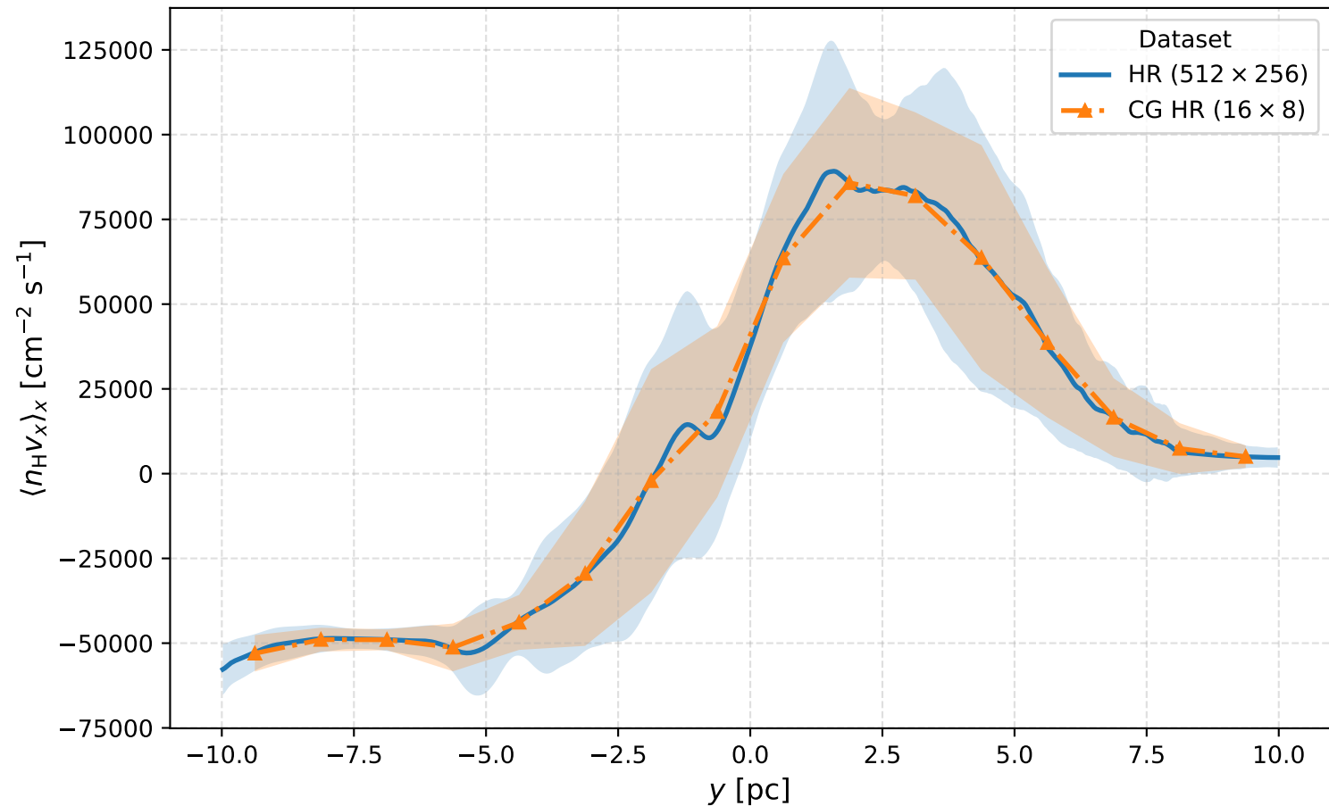
Horizontal Flux Profile \langle n_{\text{H}} v_x \rangle_x (Time-averaged over last 500 snapshots, showing mean \pm 1\sigma across time)
