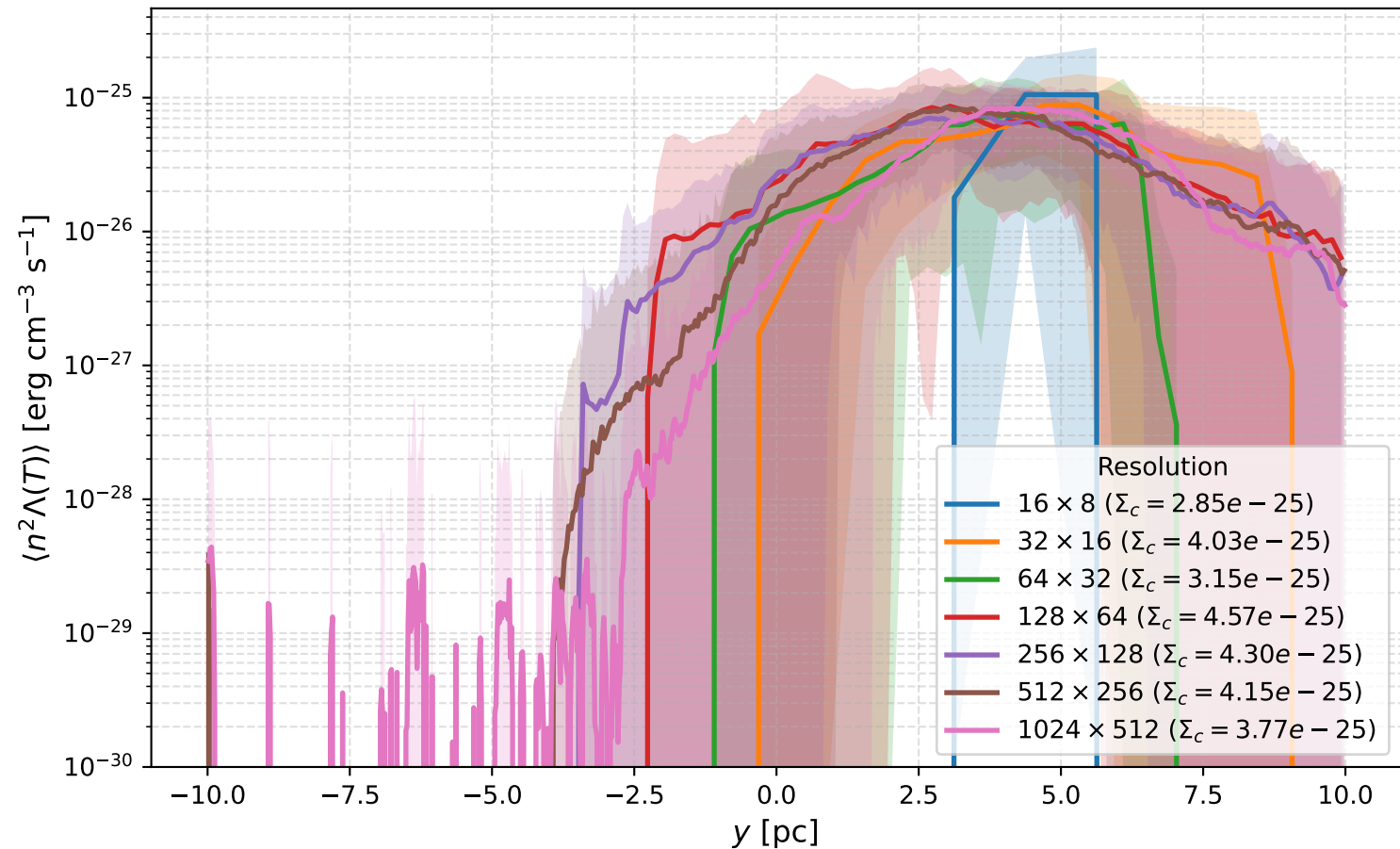
Mean Cooling Rate Profile vs y (Time-averaged over last 500 snapshots, showing mean \pm 1\sigma across time)
