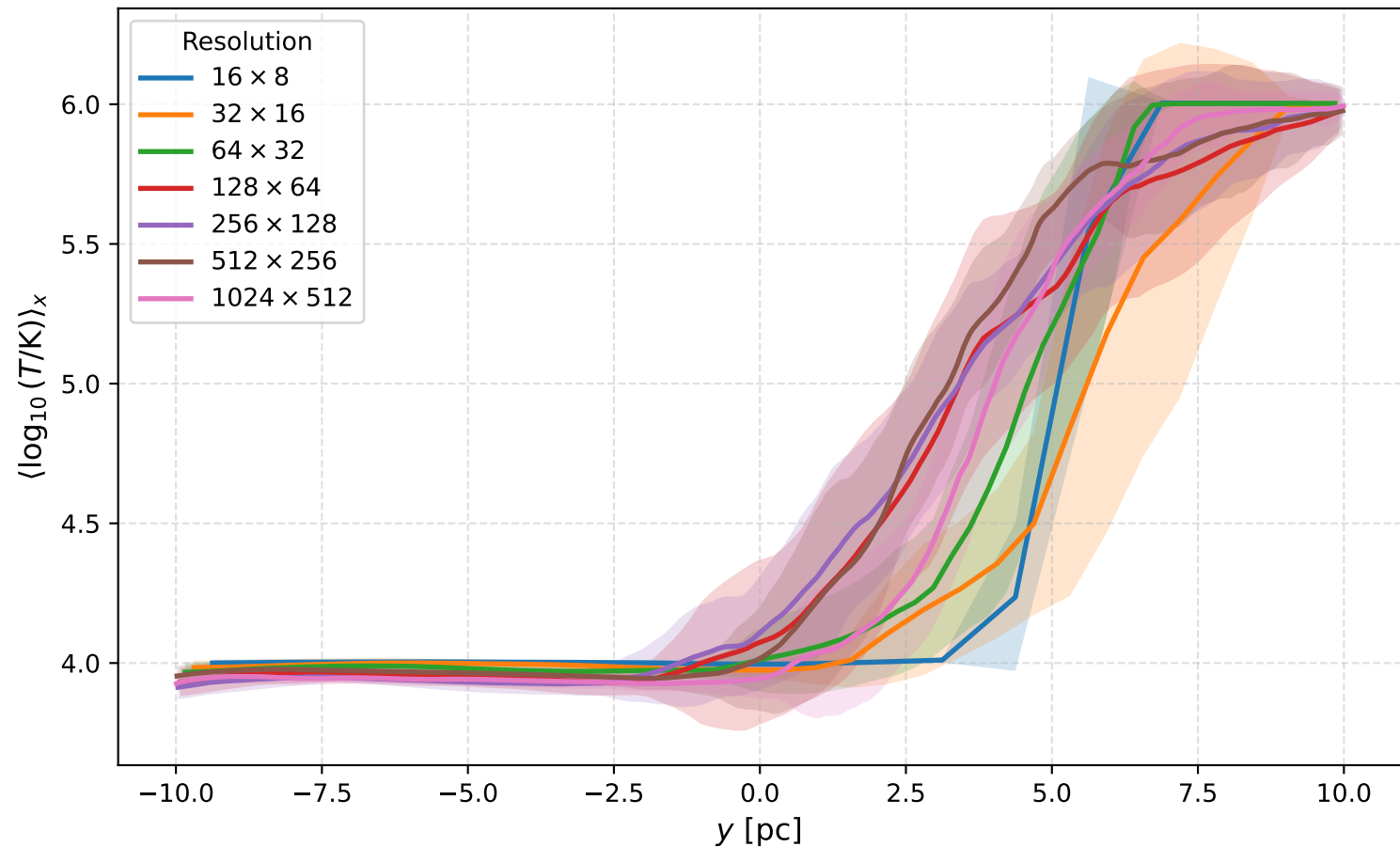
Log-Temperature Profile \langle \log_{10} T \rangle_x
