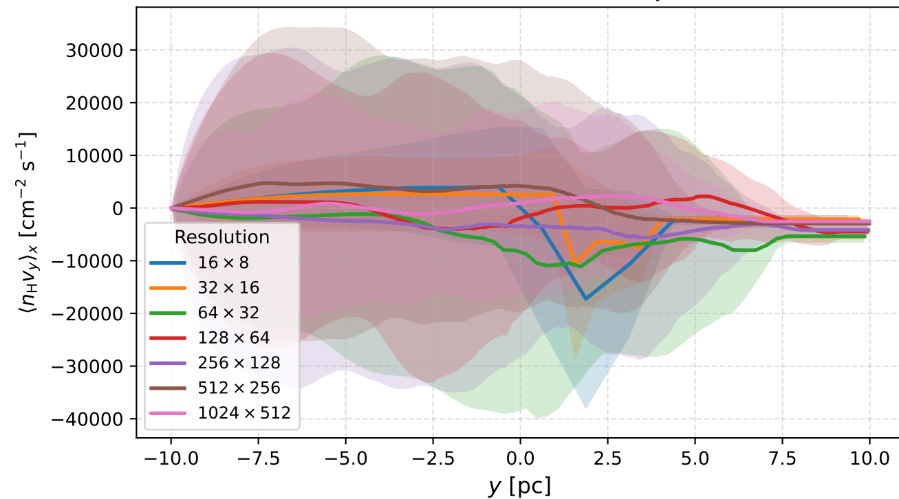
Vertical Flux Profile \langle n_H v_y \rangle_x
