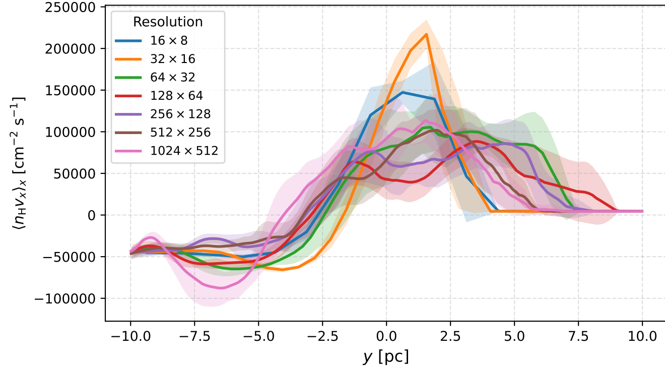
Horizontal Flux Profile \langle n_H v_x \rangle_x
