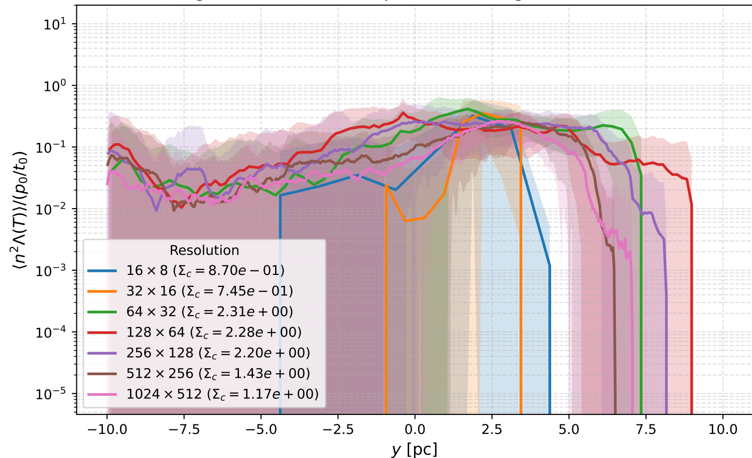
Normalized Cooling Rate \langle n^2 \Lambda(T) \rangle / (p_0/t_0) vs y (Time-averaged over last 500 snapshots, showing mean \pm 1\sigma across time)
