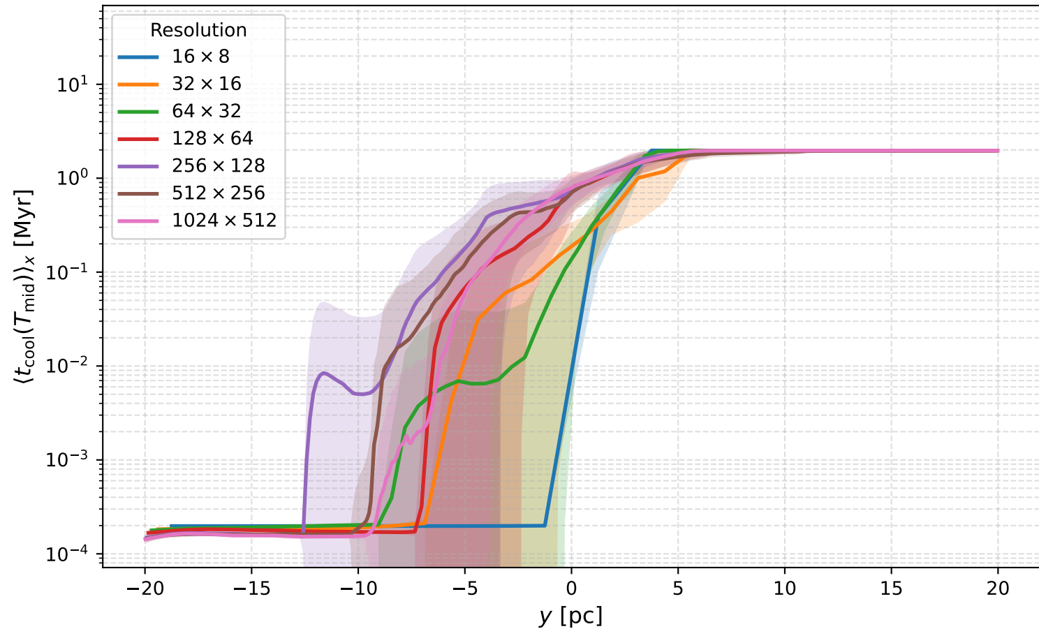
Cooling Time Profile t_{\text{cool}}(T_{\text{mid}}) vs y (Time-averaged over last 500 snapshots, showing mean \pm 1\sigma across time)
