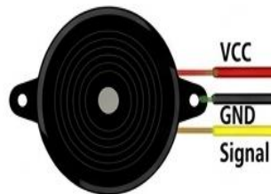
ACTIVE BUZZER
