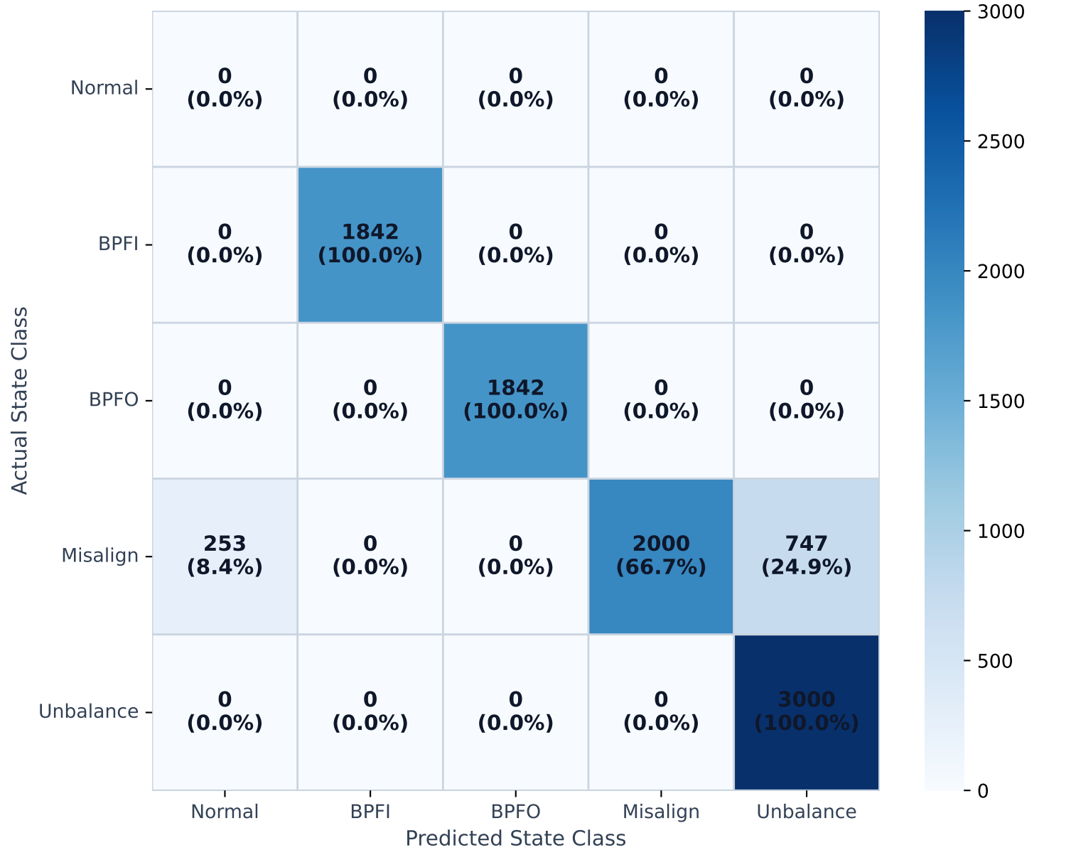
Confusion Matrix: Optimized GB + IF (Unseen Holdout Files - Strict Split)
