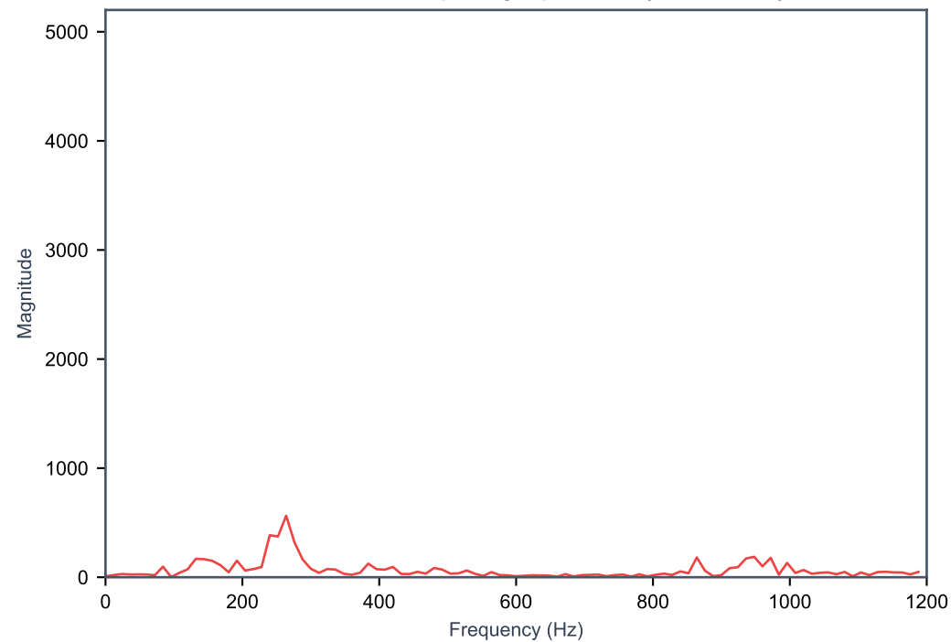
BPFO Fault: Frequency Spectrum (Harmonics)
