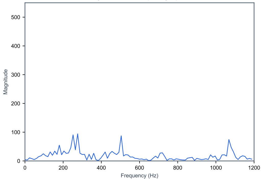
Healthy Machine: Frequency Spectrum
