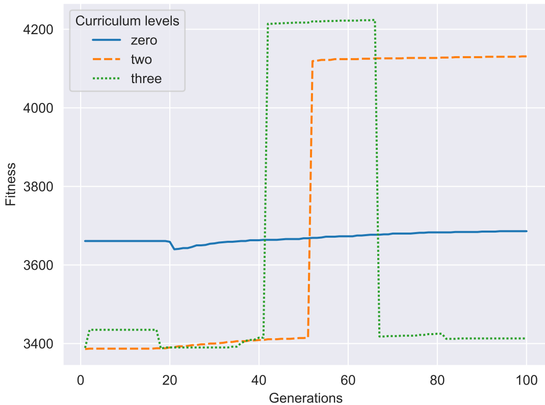
Highest fitness in each generation
