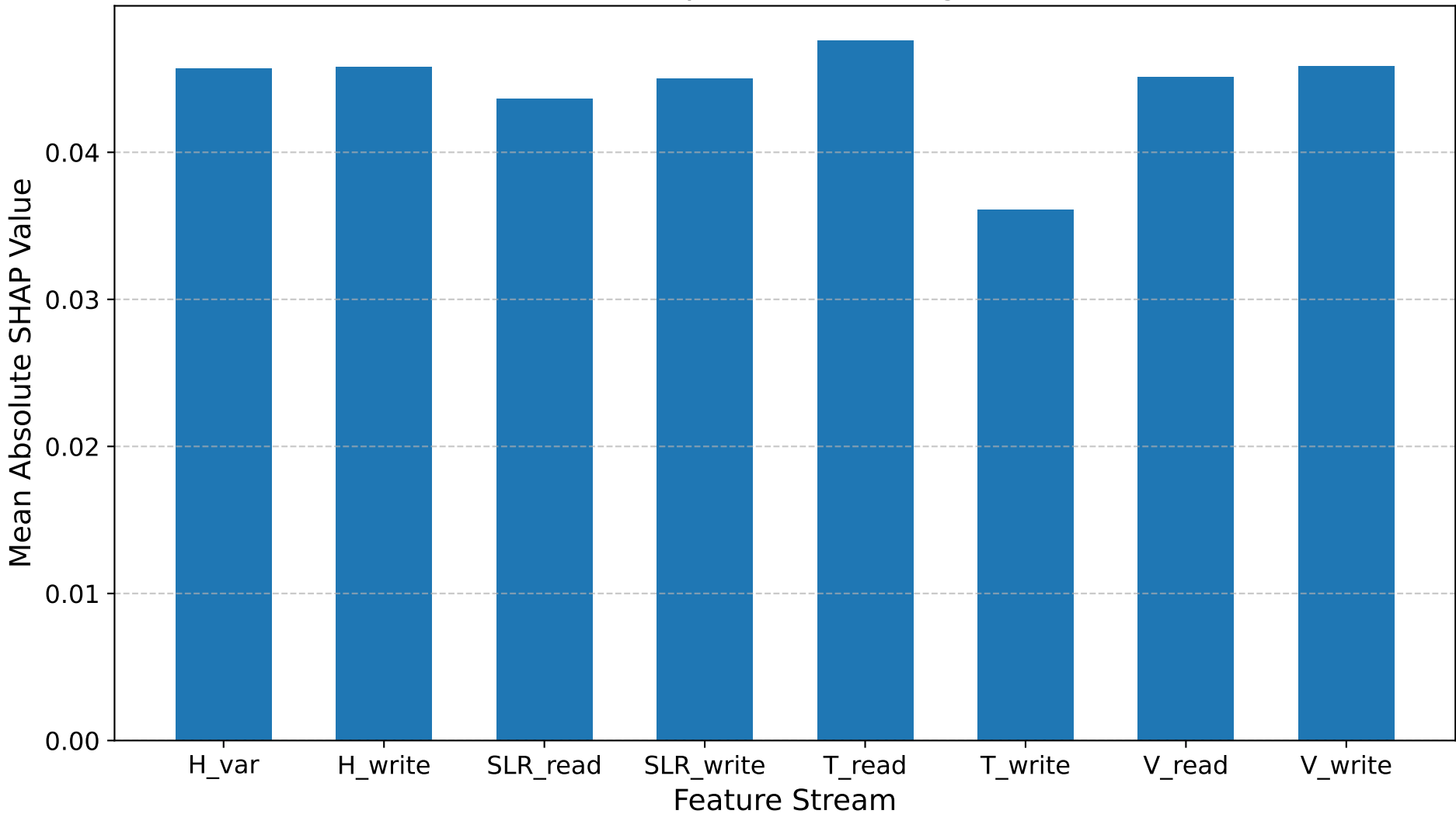
Global SHAP Feature Importance Averaged Over All Classes
