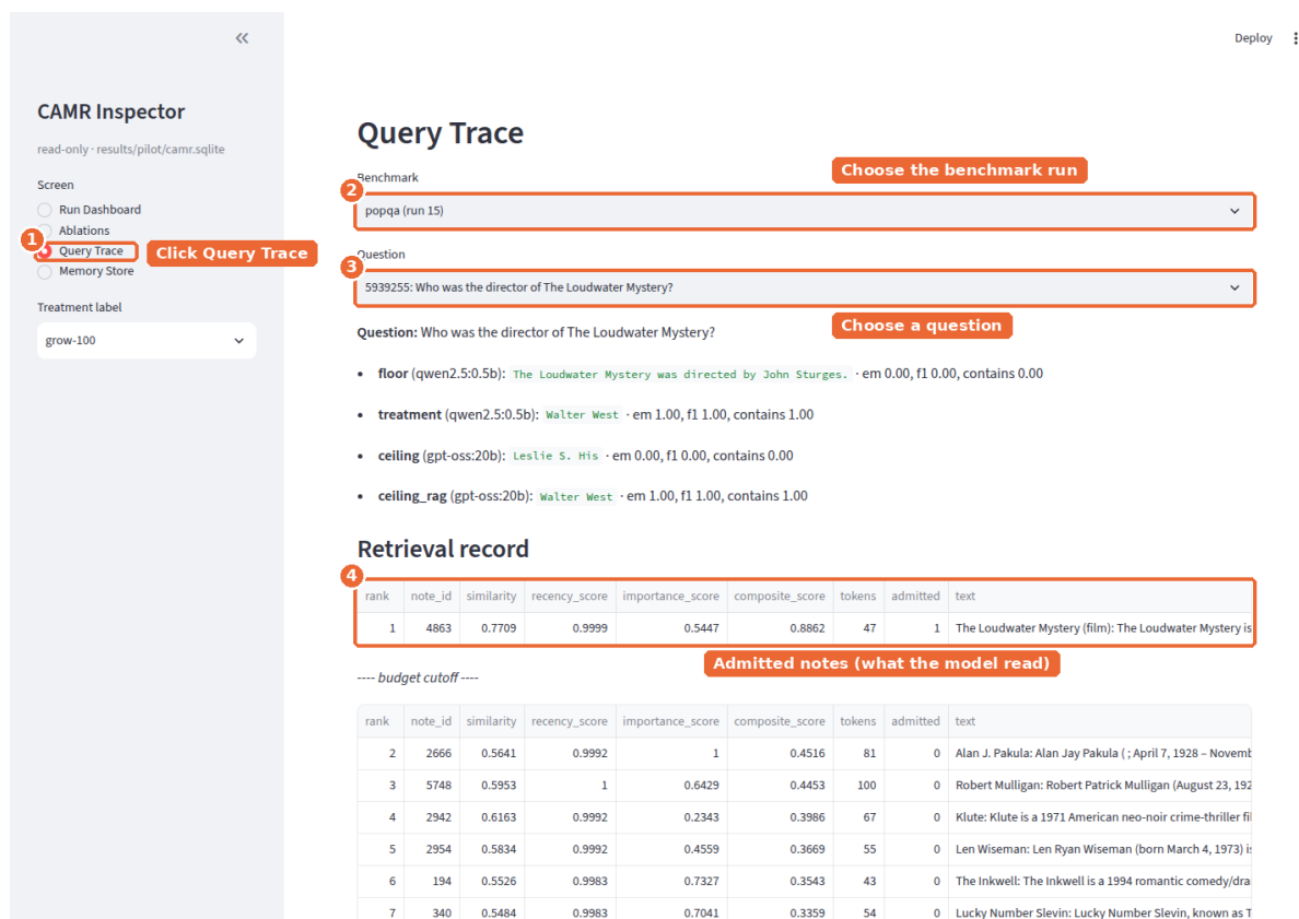
Figure 5.4: Query Trace for one PopQA question at full memory, showing the admitted note and the budget cutoff
