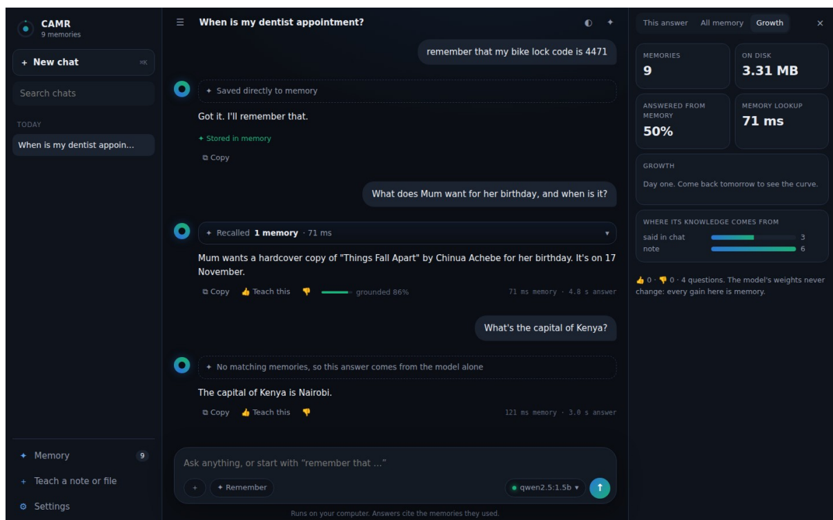
Figure 5.10: CAMR Personal: the growth panel (memories, share of answers drawn from memory, lookup time, sources of knowledge)
