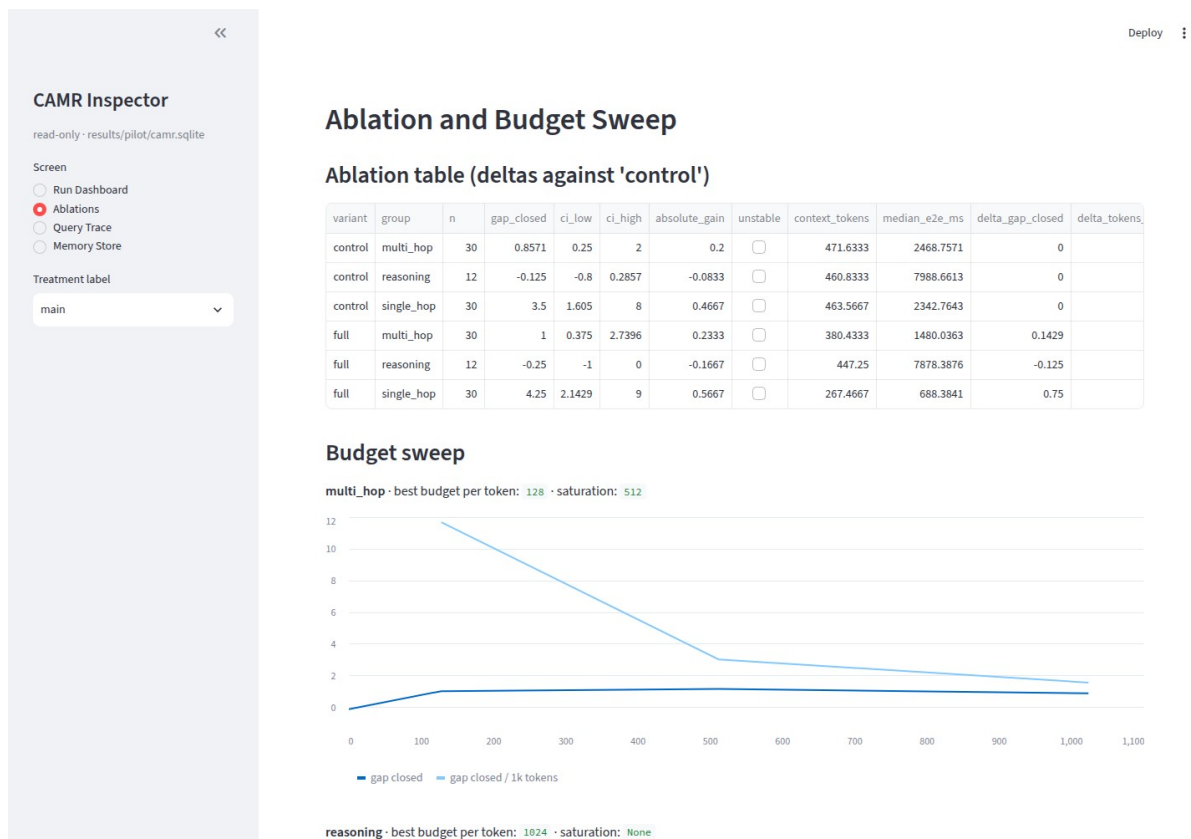
Figure 5.5: Ablations and budget-sweep screen
