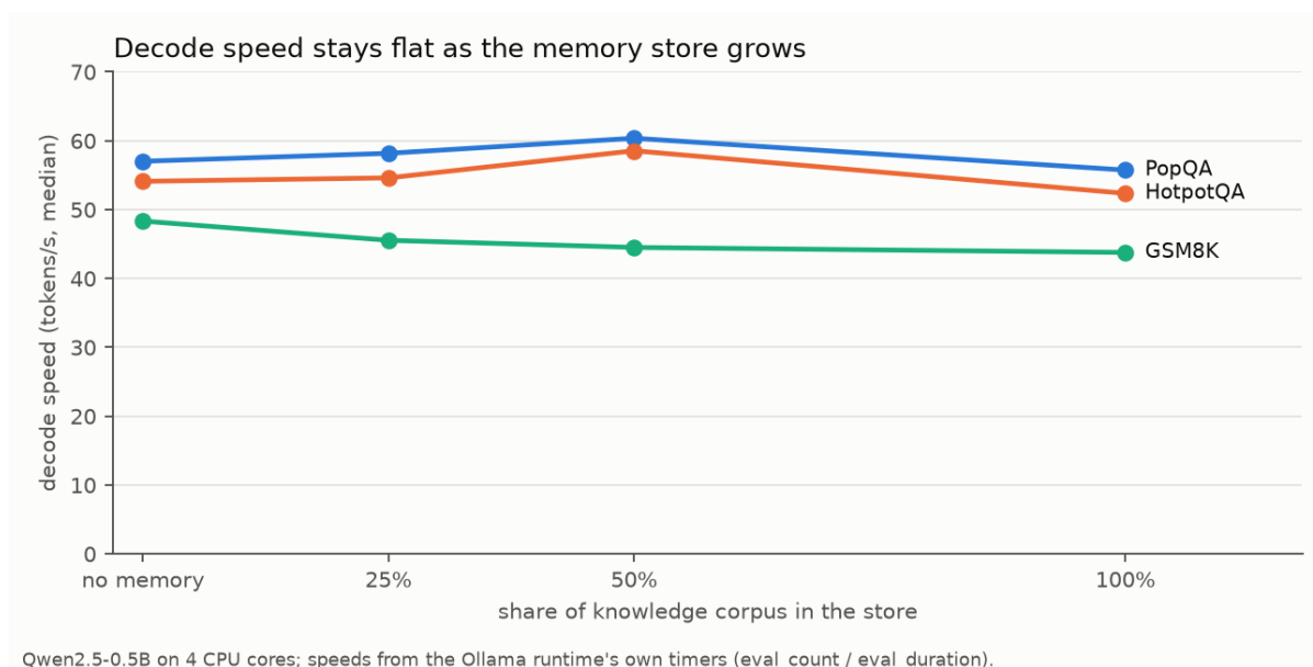
Figure 5.13: Decode speed of the frozen 0.5B model at each store size
