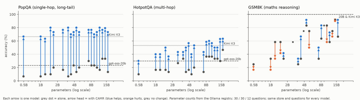
Figure 5.14: Accuracy without and with CAMR by model size, against the Kimi K3 ceiling
