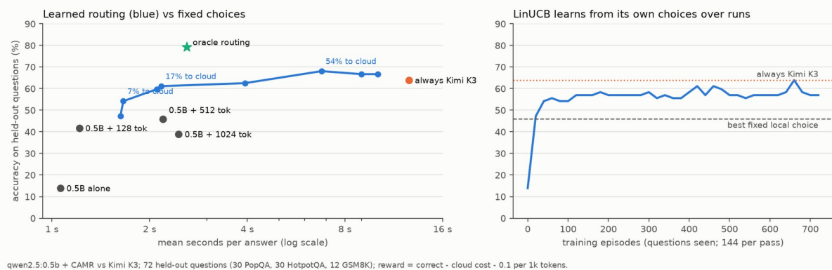
Figure 5.15: Learned routing compared with fixed choices, and the LinUCB learning curve over 5 epochs
