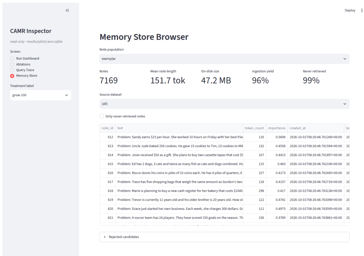
Figure 5.6: Memory Store browser: notes, provenance and retrieval counts
