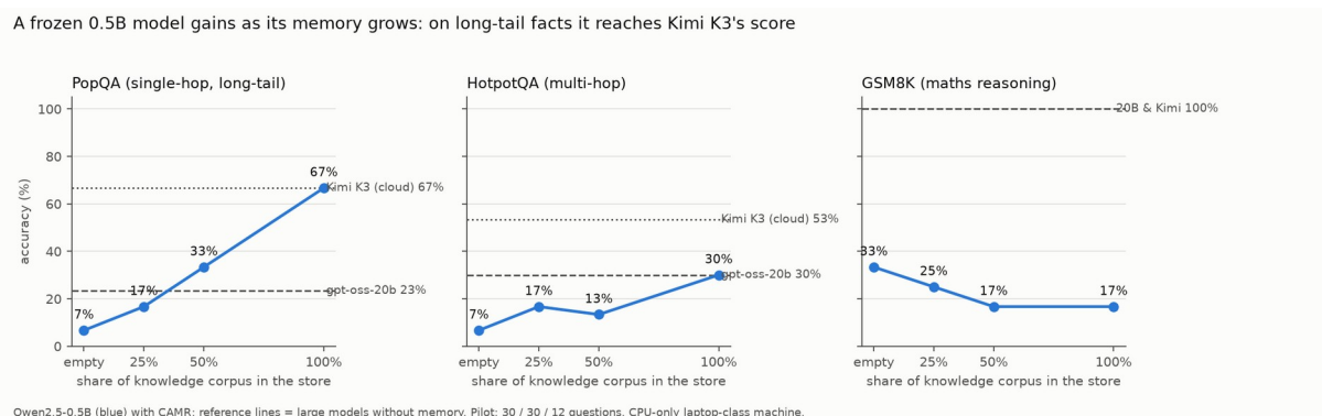
Figure 5.12: Accuracy of the frozen 0.5B model as the memory store grows
