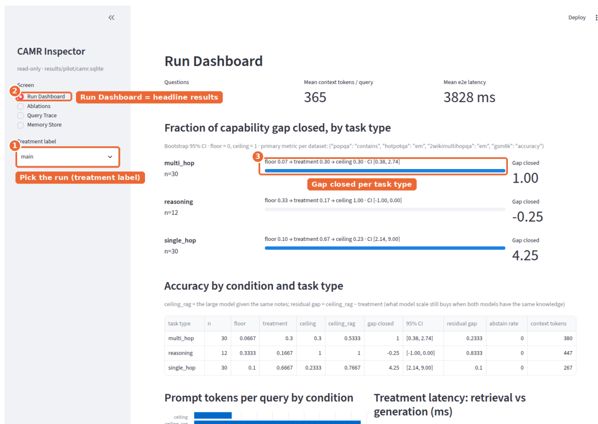
Figure 5.3: Run Dashboard of the final pilot (markers: run selector, screen, gap closed per task type)
