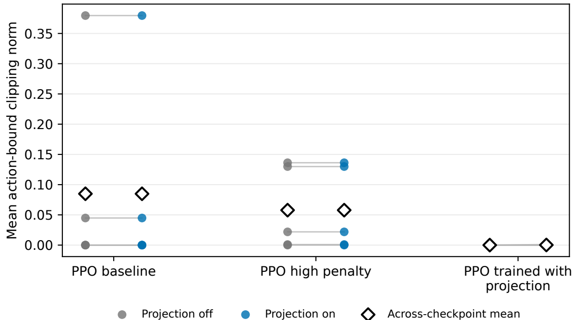
Mean action-bound clipping norm
