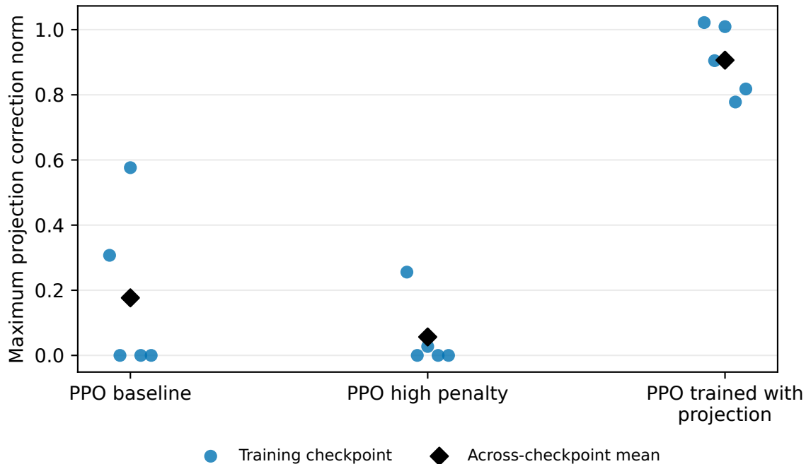
Maximum projection correction norm
