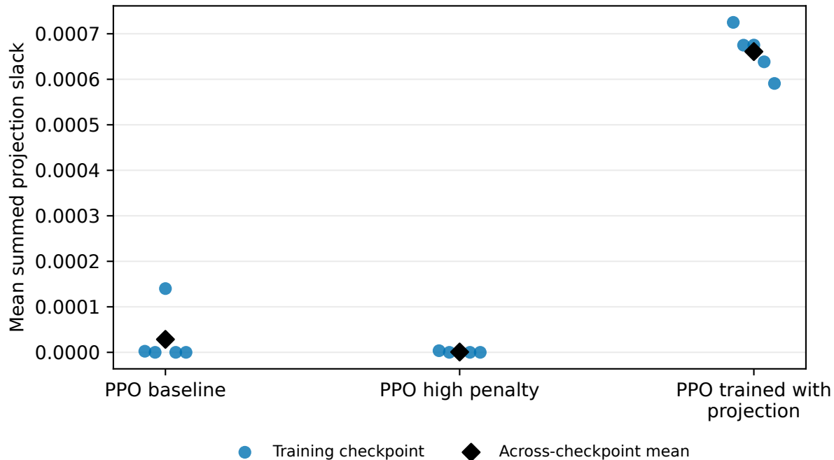
Mean summed projection slack
