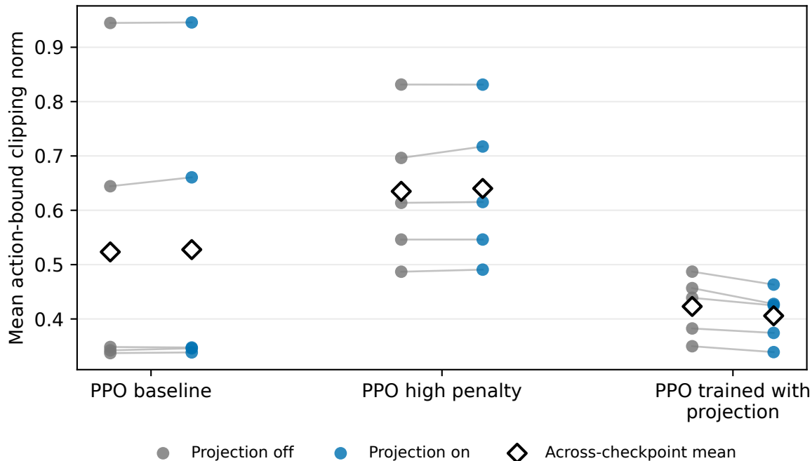
Mean action-bound clipping norm
