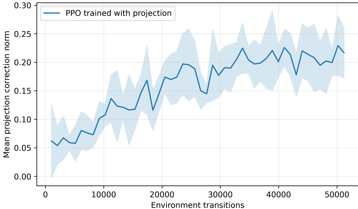
Mean projection correction norm
