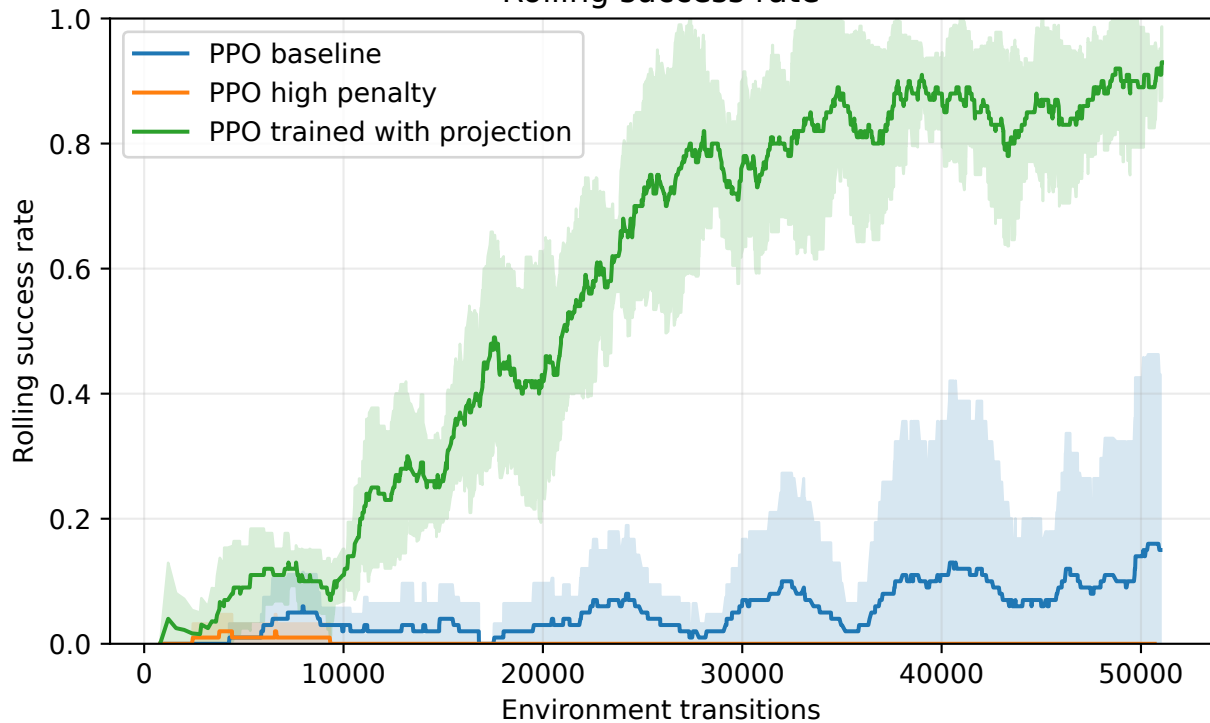
Rolling success rate
